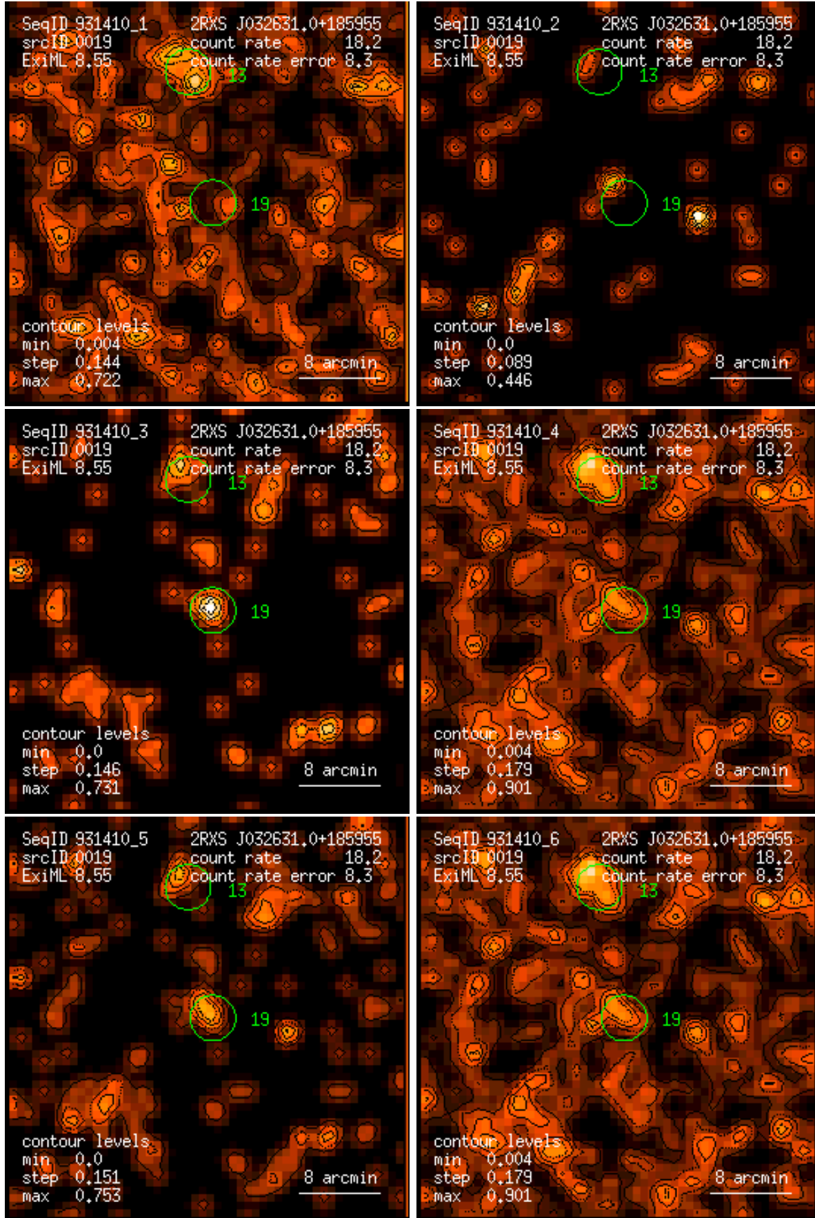
Figure 19: RASS 931410: detection 0019: band rate images, Gaussian filter: (1) PSPC channels 11 – 41, (2) 52 – 90, (3) 91 – 201, (4) 11 – 235, (5) 52 – 201, (6) 11 – 201. Broad band rates in counts/ks. Band rate contour levels in counts/ks/arcmin 2 .
