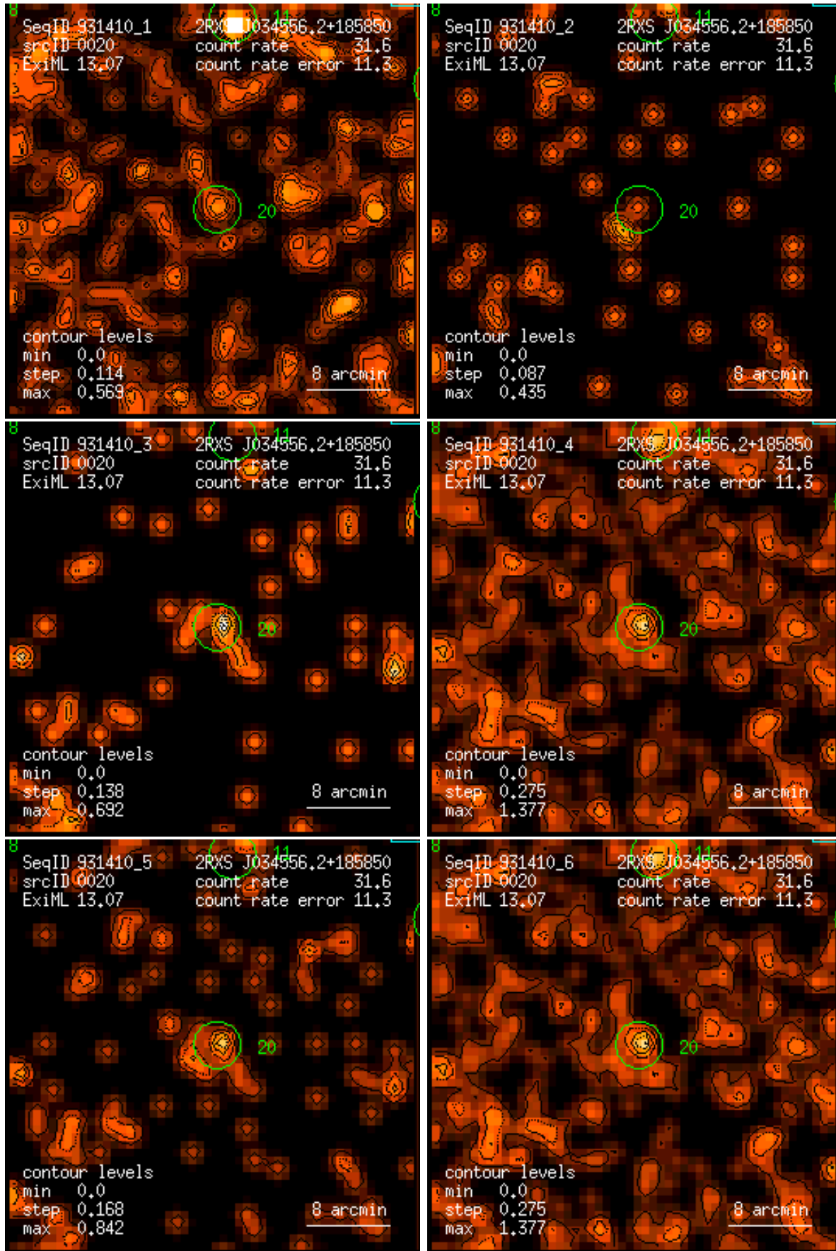
Figure 20: RASS 931410: detection 0020: band rate images, Gaussian filter: (1) PSPC channels 11 – 41, (2) 52 – 90, (3) 91 – 201, (4) 11 – 235, (5) 52 – 201, (6) 11 – 201. Broad band rates in counts/ks. Band rate contour levels in counts/ks/arcmin 2 .
