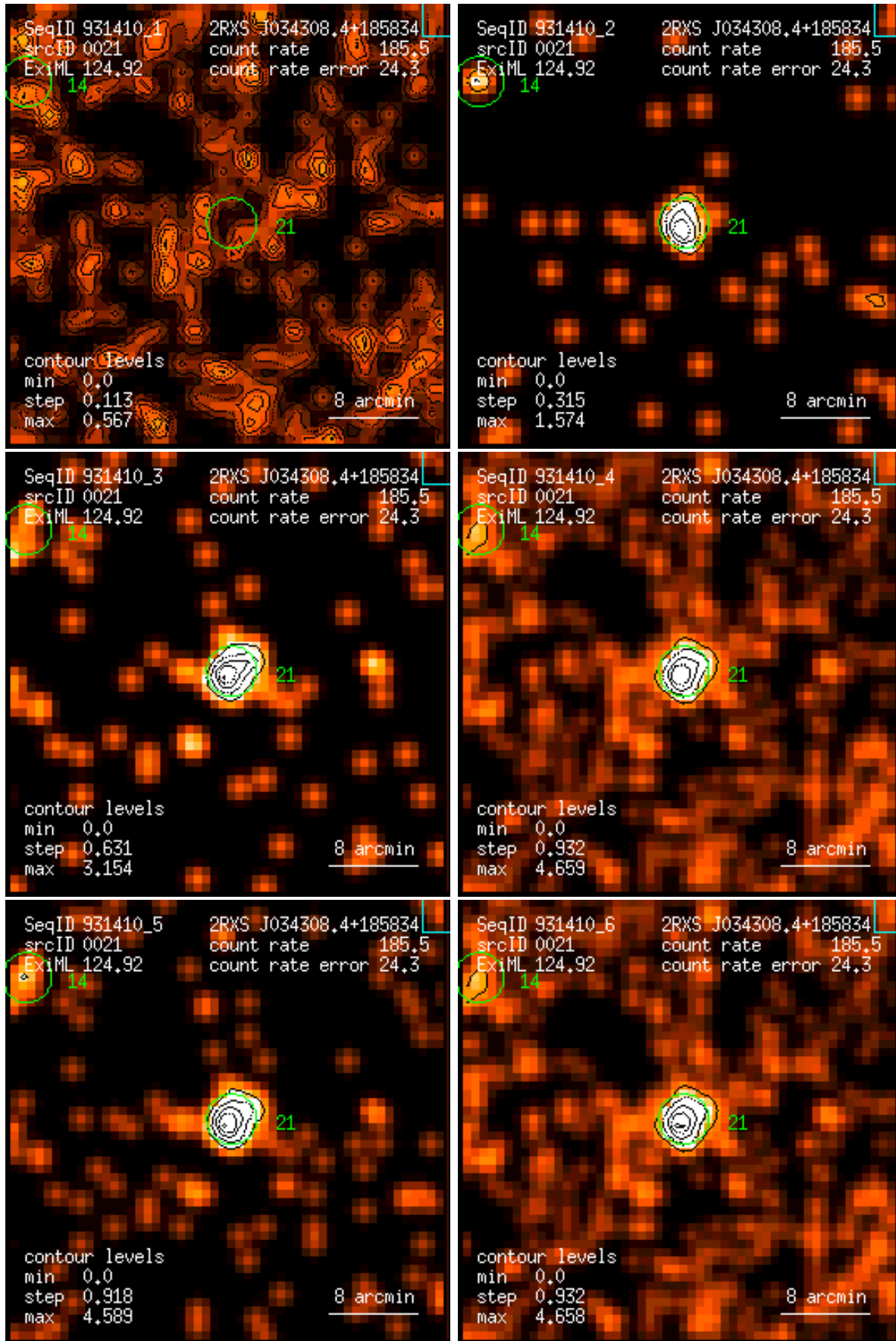
Figure 21: RASS 931410: detection 0021: band rate images, Gaussian filter: (1) PSPC channels 11 – 41, (2) 52 – 90, (3) 91 – 201, (4) 11 – 235, (5) 52 – 201, (6) 11 – 201. Broad band rates in counts/ks. Band rate contour levels in counts/ks/arcmin 2 .
