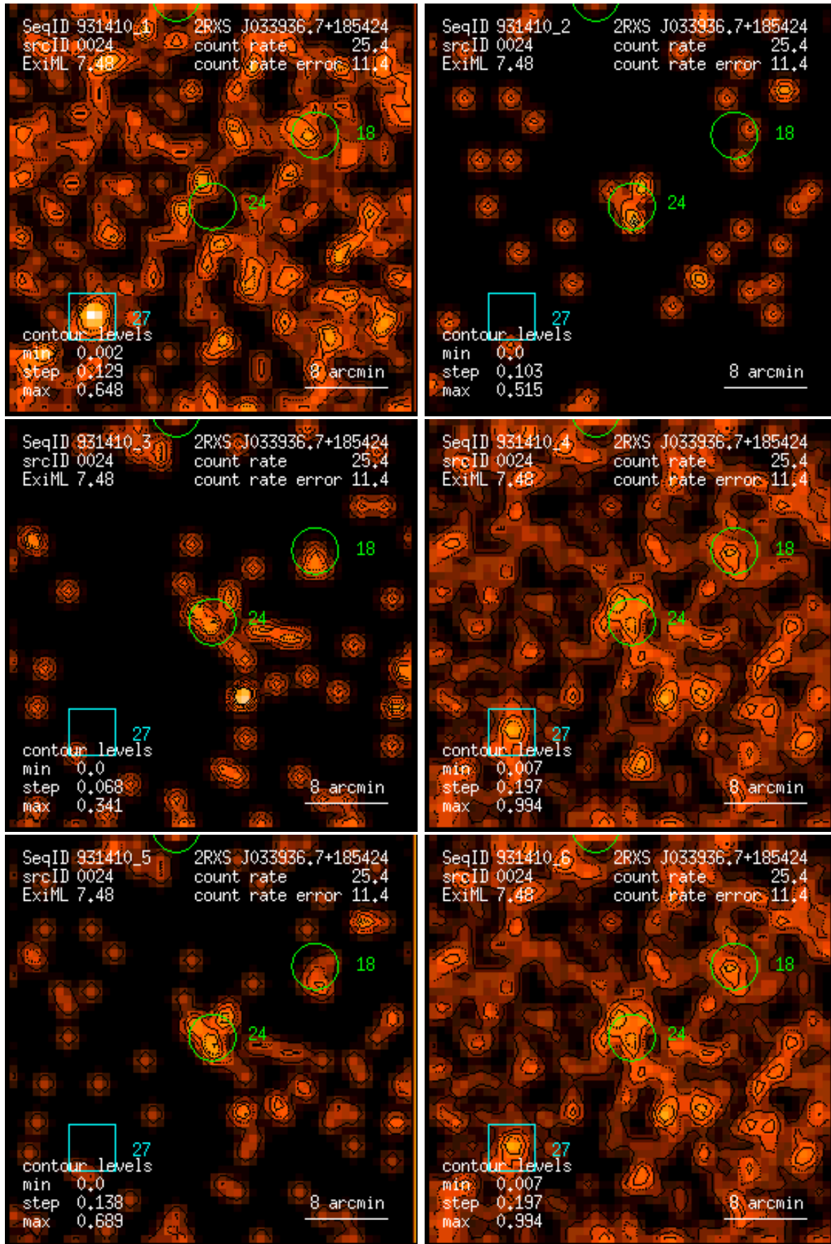
Figure 24: RASS 931410: detection 0024: band rate images, Gaussian filter: (1) PSPC channels 11 – 41, (2) 52 – 90, (3) 91 – 201, (4) 11 – 235, (5) 52 – 201, (6) 11 – 201. Broad band rates in counts/ks. Band rate contour levels in counts/ks/arcmin 2 .
