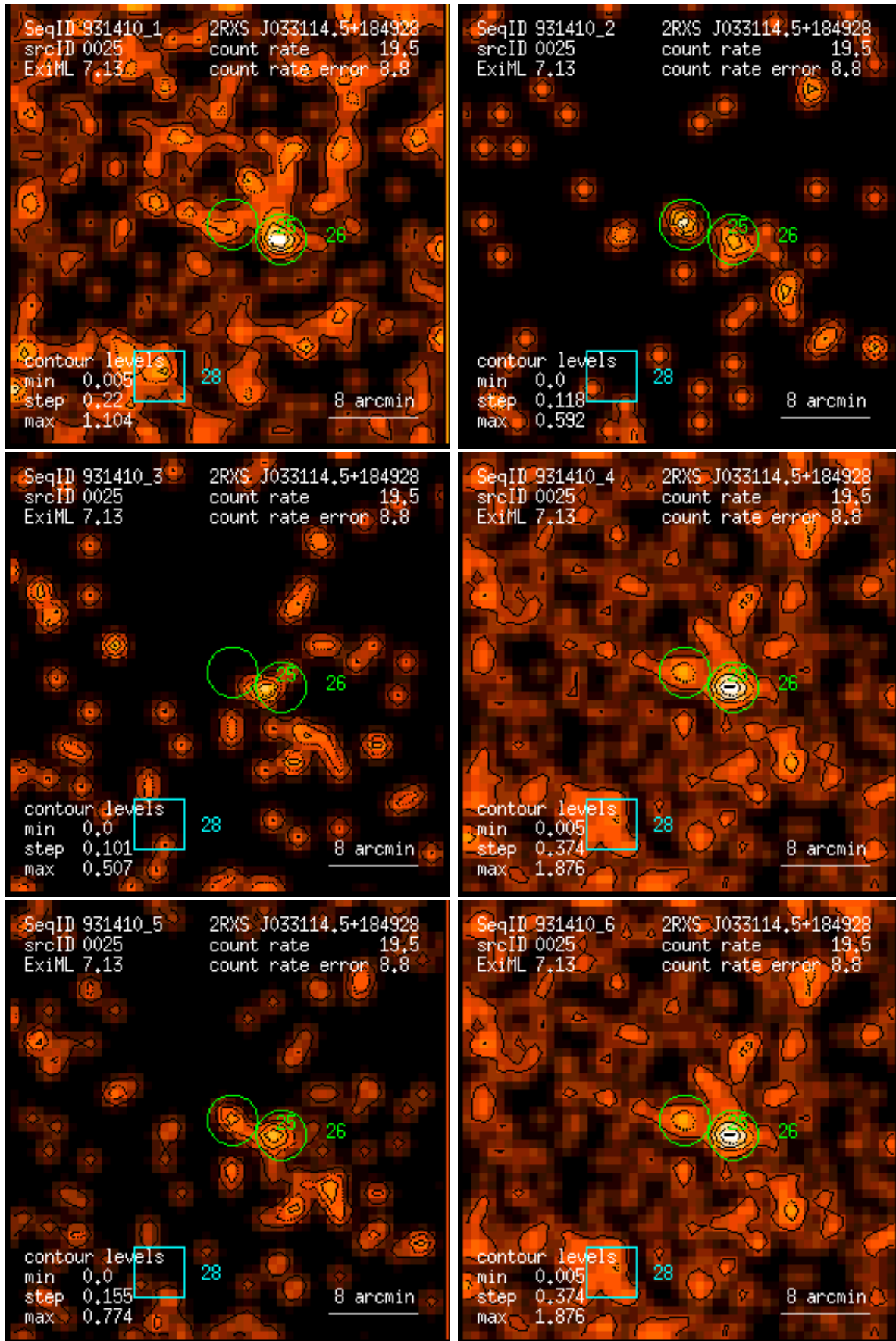
Figure 25: RASS 931410: detection 0025: band rate images, Gaussian filter: (1) PSPC channels 11 – 41, (2) 52 – 90, (3) 91 – 201, (4) 11 – 235, (5) 52 – 201, (6) 11 – 201. Broad band rates in counts/ks. Band rate contour levels in counts/ks/arcmin 2 .
