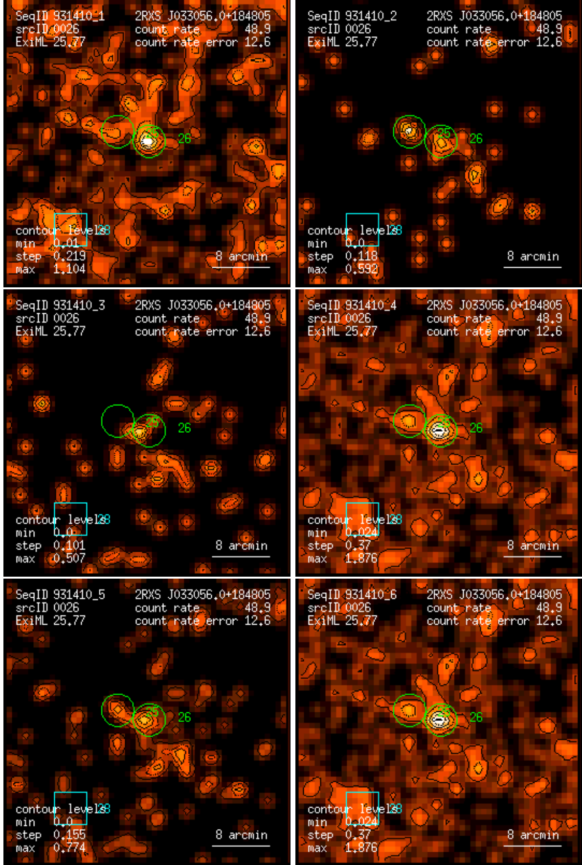
Figure 26: RASS 931410: detection 0026: band rate images, Gaussian filter: (1) PSPC channels 11 – 41, (2) 52 – 90, (3) 91 – 201, (4) 11 – 235, (5) 52 – 201, (6) 11 – 201. Broad band rates in counts/ks. Band rate contour levels in counts/ks/arcmin 2 .
