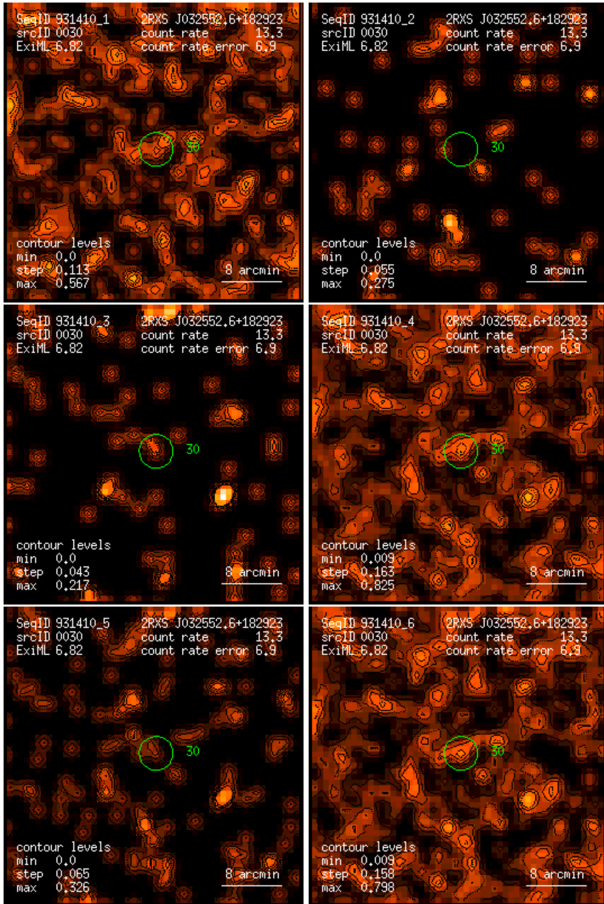
Figure 30: RASS 931410: detection 0030: band rate images, Gaussian filter: (1) PSPC channels 11 – 41, (2) 52 – 90, (3) 91 – 201, (4) 11 – 235, (5) 52 – 201, (6) 11 – 201. Broad band rates in counts/ks. Band rate contour levels in counts/ks/arcmin 2 .
