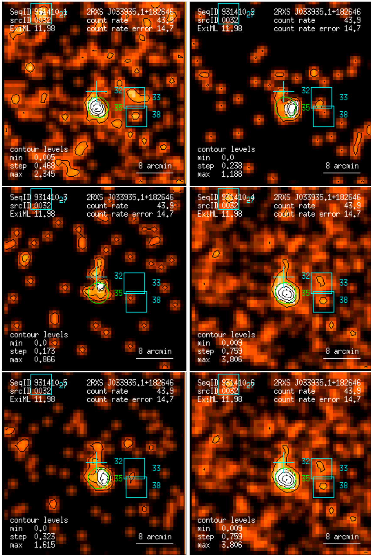
Figure 32: RASS 931410: detection 0032: band rate images, Gaussian filter: (1) PSPC channels 11 – 41, (2) 52 – 90, (3) 91 – 201, (4) 11 – 235, (5) 52 – 201, (6) 11 – 201. Broad band rates in counts/ks. Band rate contour levels in counts/ks/arcmin 2 .
