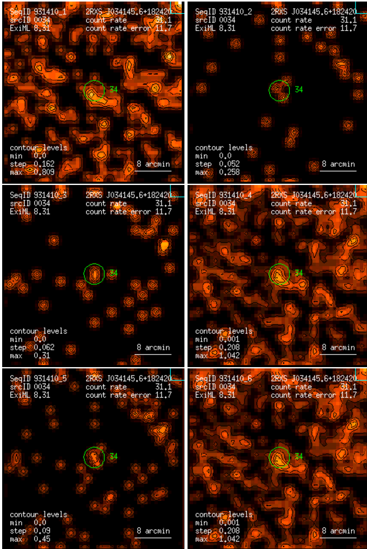
Figure 34: RASS 931410: detection 0034: band rate images, Gaussian filter: (1) PSPC channels 11 – 41, (2) 52 – 90, (3) 91 – 201, (4) 11 – 235, (5) 52 – 201, (6) 11 – 201. Broad band rates in counts/ks. Band rate contour levels in counts/ks/arcmin 2 .
