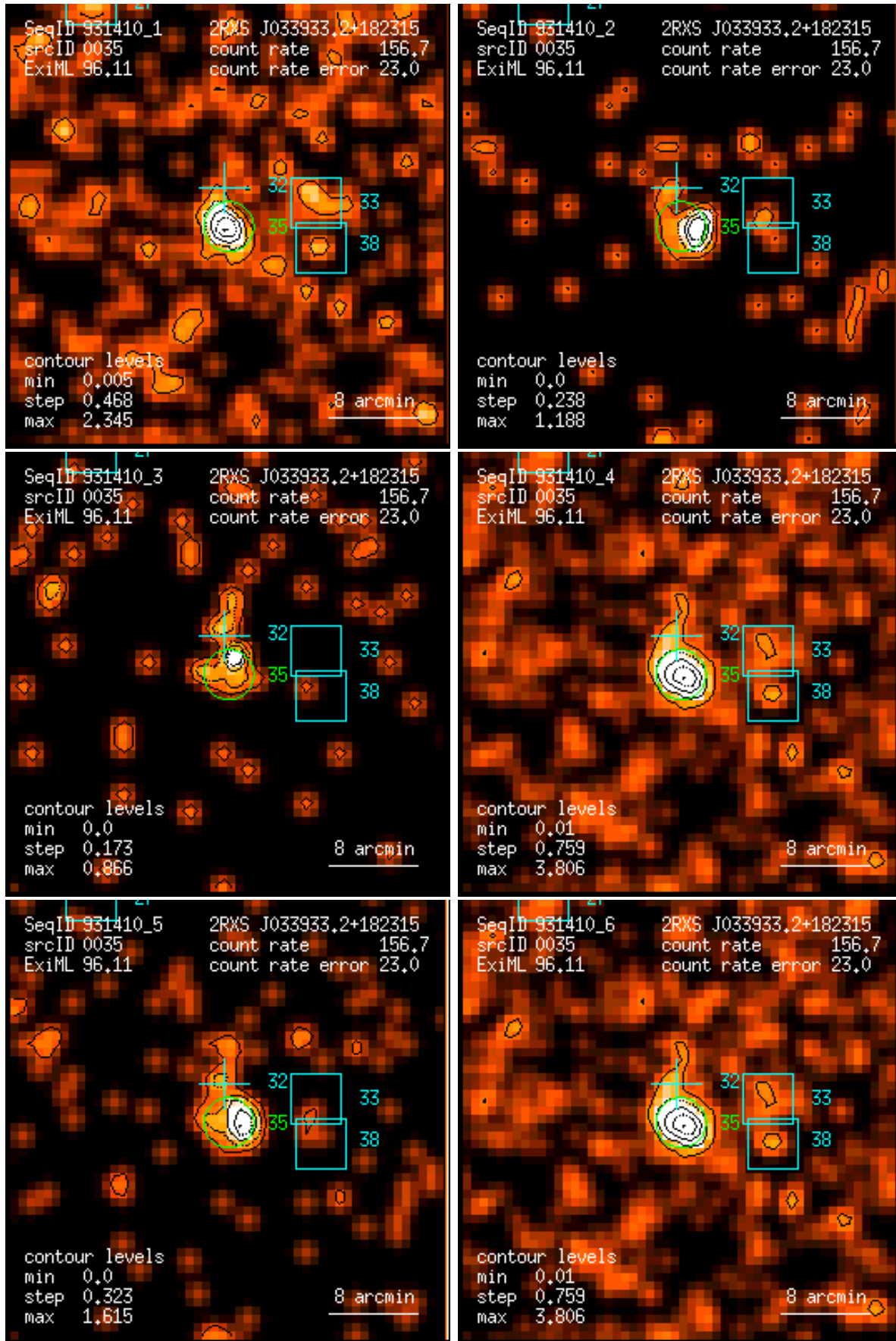
Figure 35: RASS 931410: detection 0035: band rate images, Gaussian filter: (1) PSPC channels 11 – 41, (2) 52 – 90, (3) 91 – 201, (4) 11 – 235, (5) 52 – 201, (6) 11 – 201. Broad band rates in counts/ks. Band rate contour levels in counts/ks/arcmin 2 .
