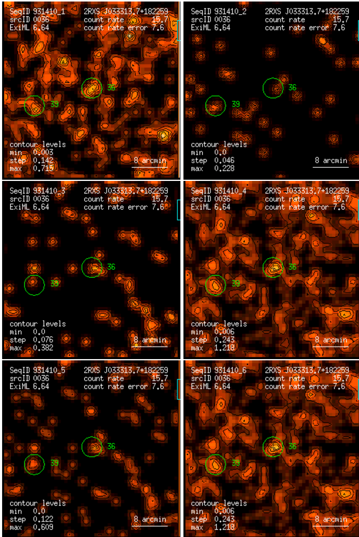
Figure 36: RASS 931410: detection 0036: band rate images, Gaussian filter: (1) PSPC channels 11 – 41, (2) 52 – 90, (3) 91 – 201, (4) 11 – 235, (5) 52 – 201, (6) 11 – 201. Broad band rates in counts/ks. Band rate contour levels in counts/ks/arcmin 2 .
