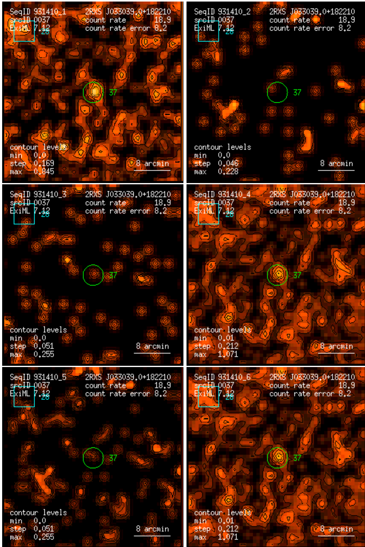
Figure 37: RASS 931410: detection 0037: band rate images, Gaussian filter: (1) PSPC channels 11 – 41, (2) 52 – 90, (3) 91 – 201, (4) 11 – 235, (5) 52 – 201, (6) 11 – 201. Broad band rates in counts/ks. Band rate contour levels in counts/ks/arcmin 2 .
