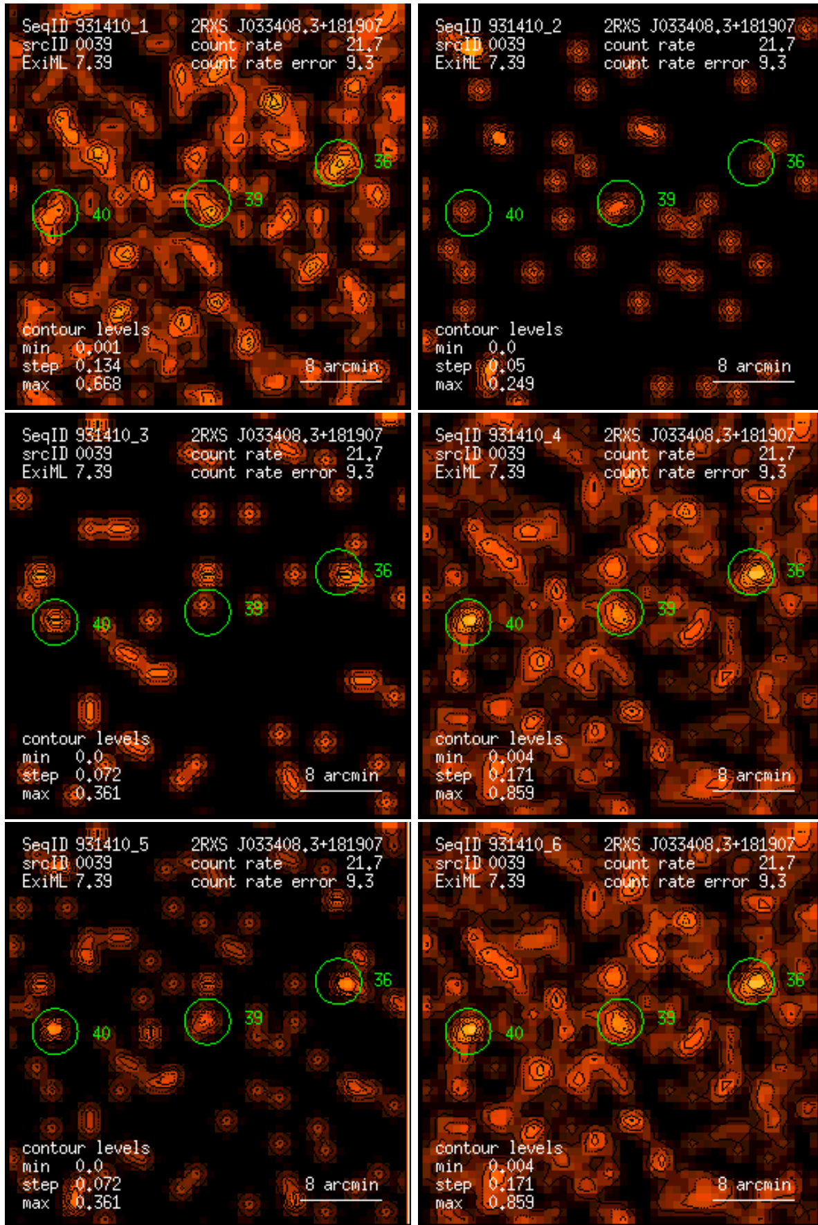
Figure 39: RASS 931410: detection 0039: band rate images, Gaussian filter: (1) PSPC channels 11 – 41, (2) 52 – 90, (3) 91 – 201, (4) 11 – 235, (5) 52 – 201, (6) 11 – 201. Broad band rates in counts/ks. Band rate contour levels in counts/ks/arcmin 2 .
