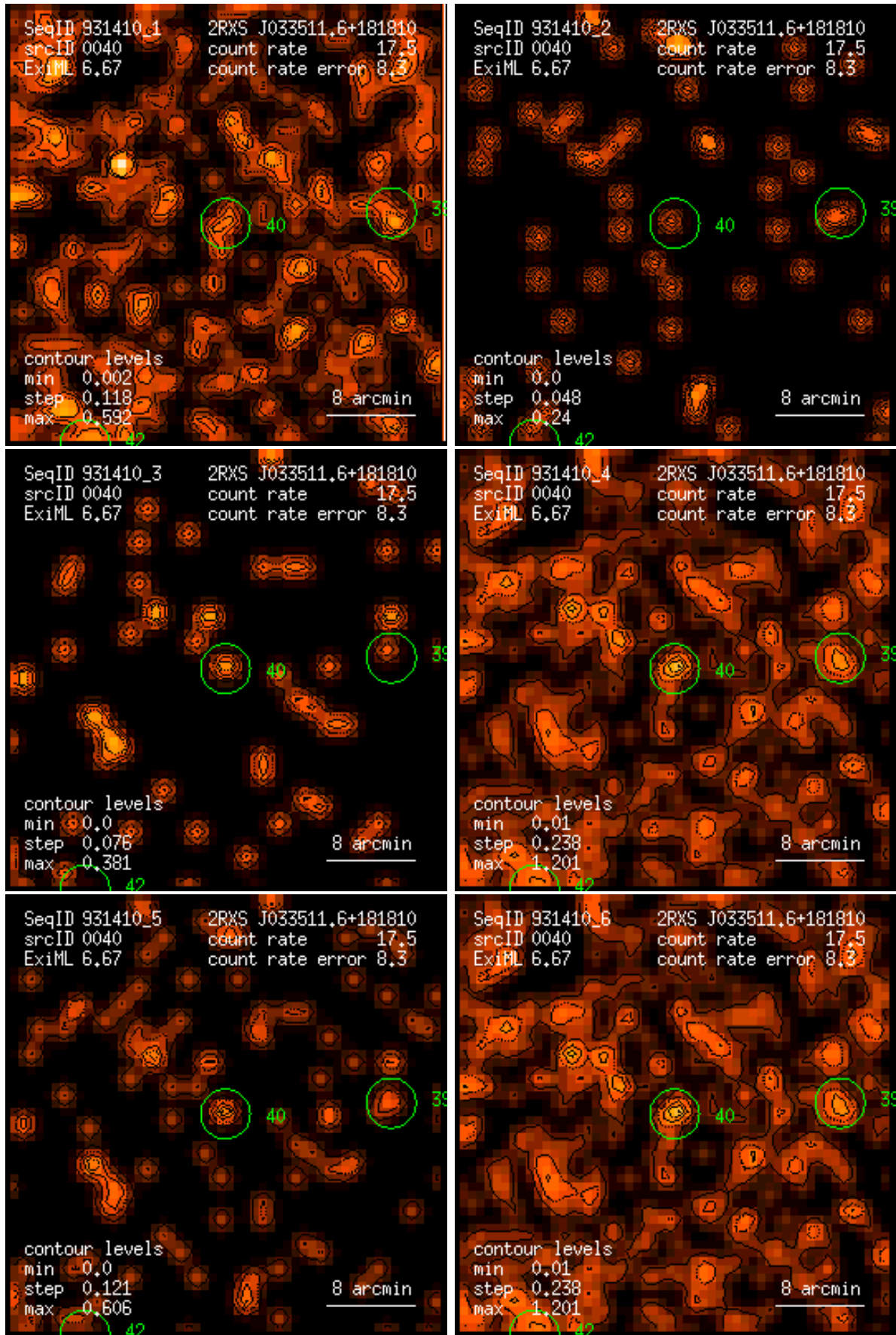
Figure 40: RASS 931410: detection 0040: band rate images, Gaussian filter: (1) PSPC channels 11 – 41, (2) 52 – 90, (3) 91 – 201, (4) 11 – 235, (5) 52 – 201, (6) 11 – 201. Broad band rates in counts/ks. Band rate contour levels in counts/ks/arcmin 2 .
