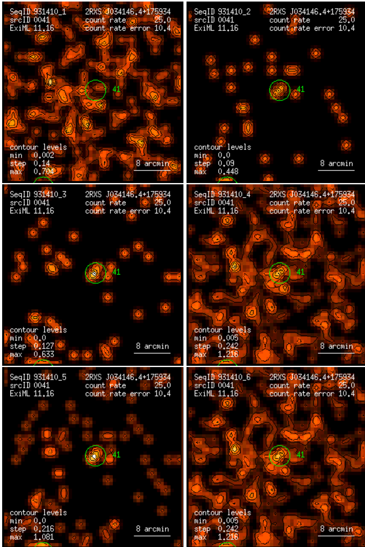
Figure 41: RASS 931410: detection 0041: band rate images, Gaussian filter: (1) PSPC channels 11 – 41, (2) 52 – 90, (3) 91 – 201, (4) 11 – 235, (5) 52 – 201, (6) 11 – 201. Broad band rates in counts/ks. Band rate contour levels in counts/ks/arcmin 2 .
