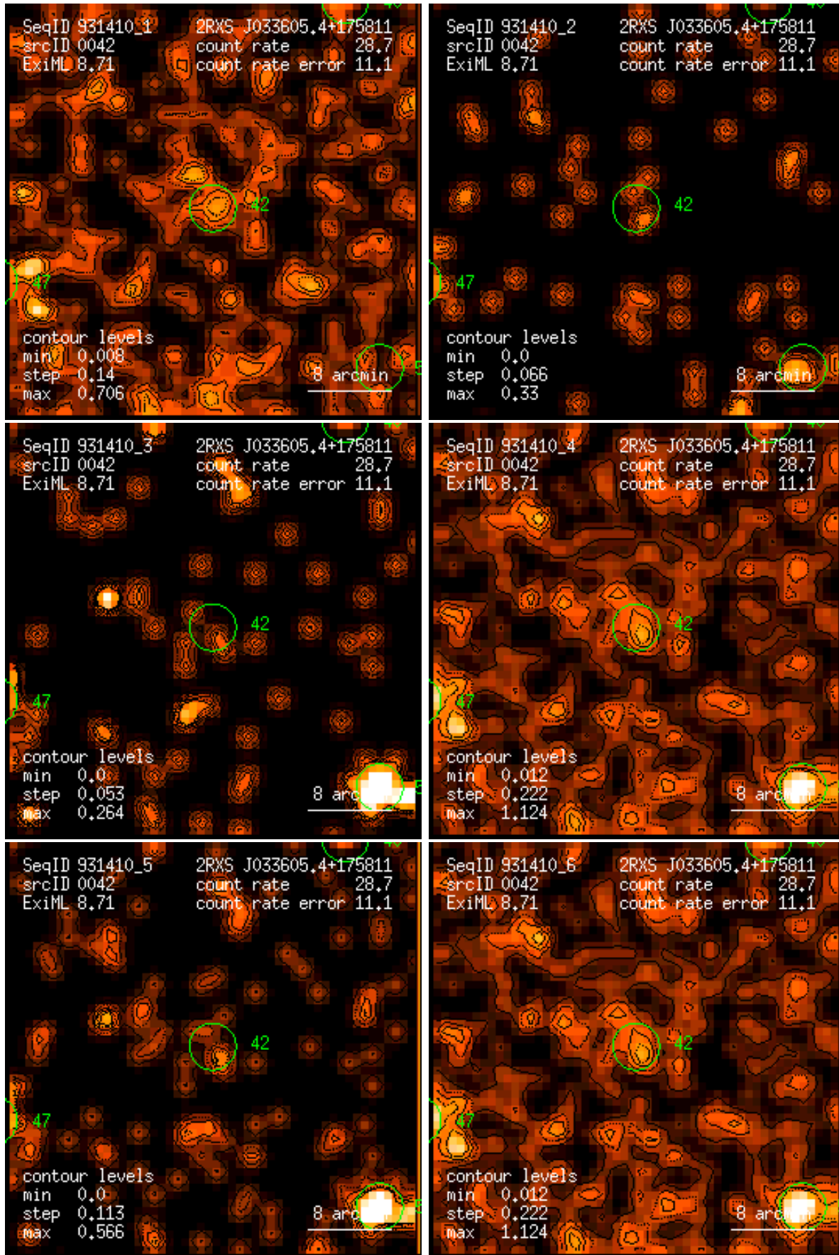
Figure 42: RASS 931410: detection 0042: band rate images, Gaussian filter: (1) PSPC channels 11 – 41, (2) 52 – 90, (3) 91 – 201, (4) 11 – 235, (5) 52 – 201, (6) 11 – 201. Broad band rates in counts/ks. Band rate contour levels in counts/ks/arcmin 2 .
