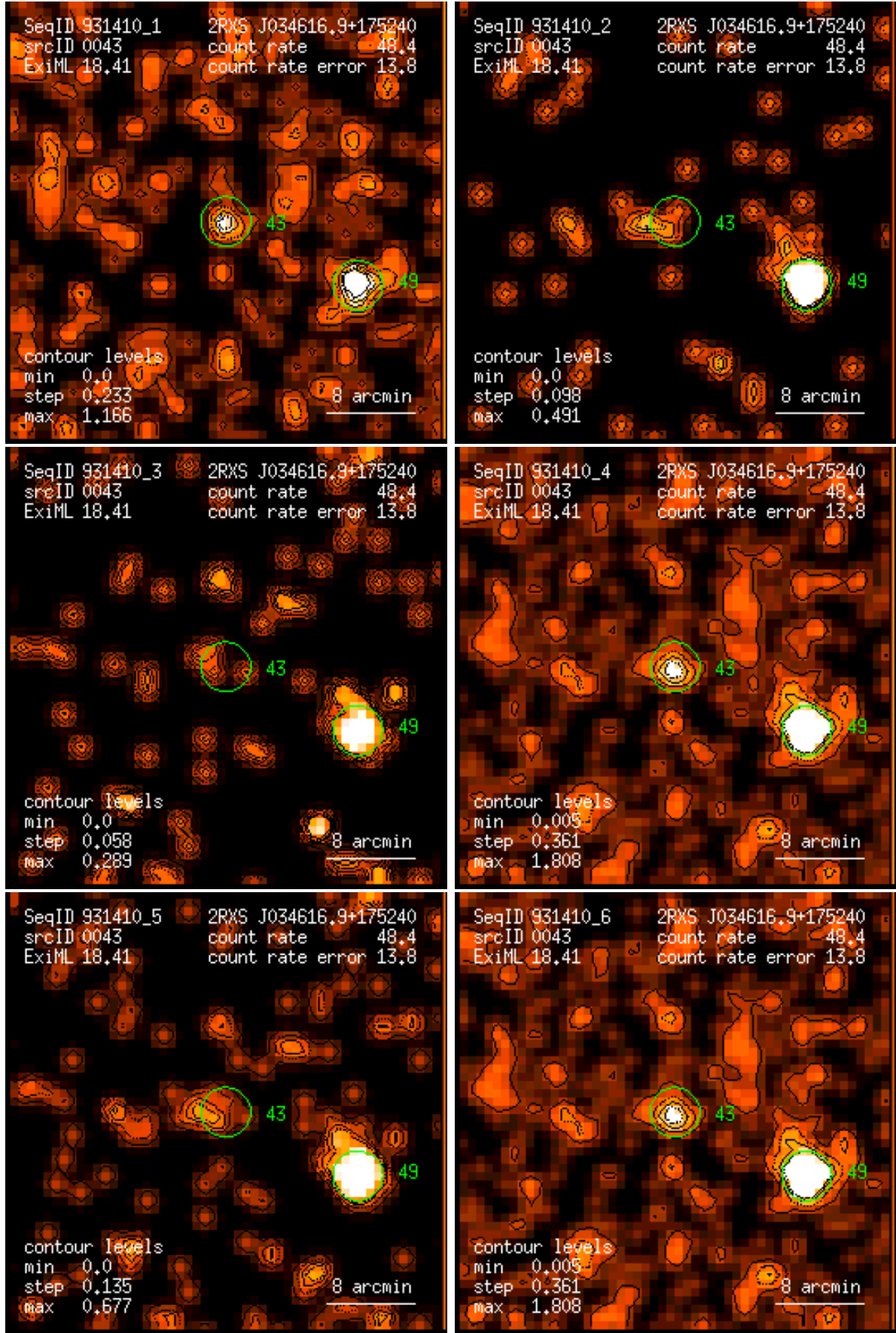
Figure 43: RASS 931410: detection 0043: band rate images, Gaussian filter: (1) PSPC channels 11 – 41, (2) 52 – 90, (3) 91 – 201, (4) 11 – 235, (5) 52 – 201, (6) 11 – 201. Broad band rates in counts/ks. Band rate contour levels in counts/ks/arcmin 2 .
