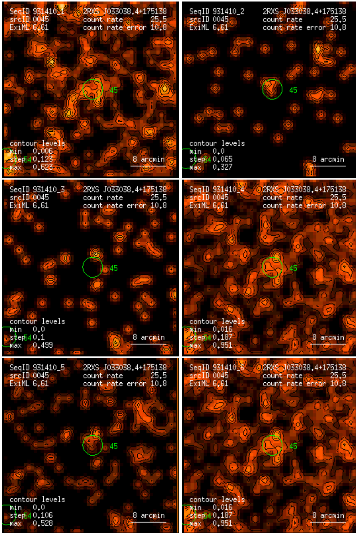
Figure 45: RASS 931410: detection 0045: band rate images, Gaussian filter: (1) PSPC channels 11 – 41, (2) 52 – 90, (3) 91 – 201, (4) 11 – 235, (5) 52 – 201, (6) 11 – 201. Broad band rates in counts/ks. Band rate contour levels in counts/ks/arcmin 2 .
