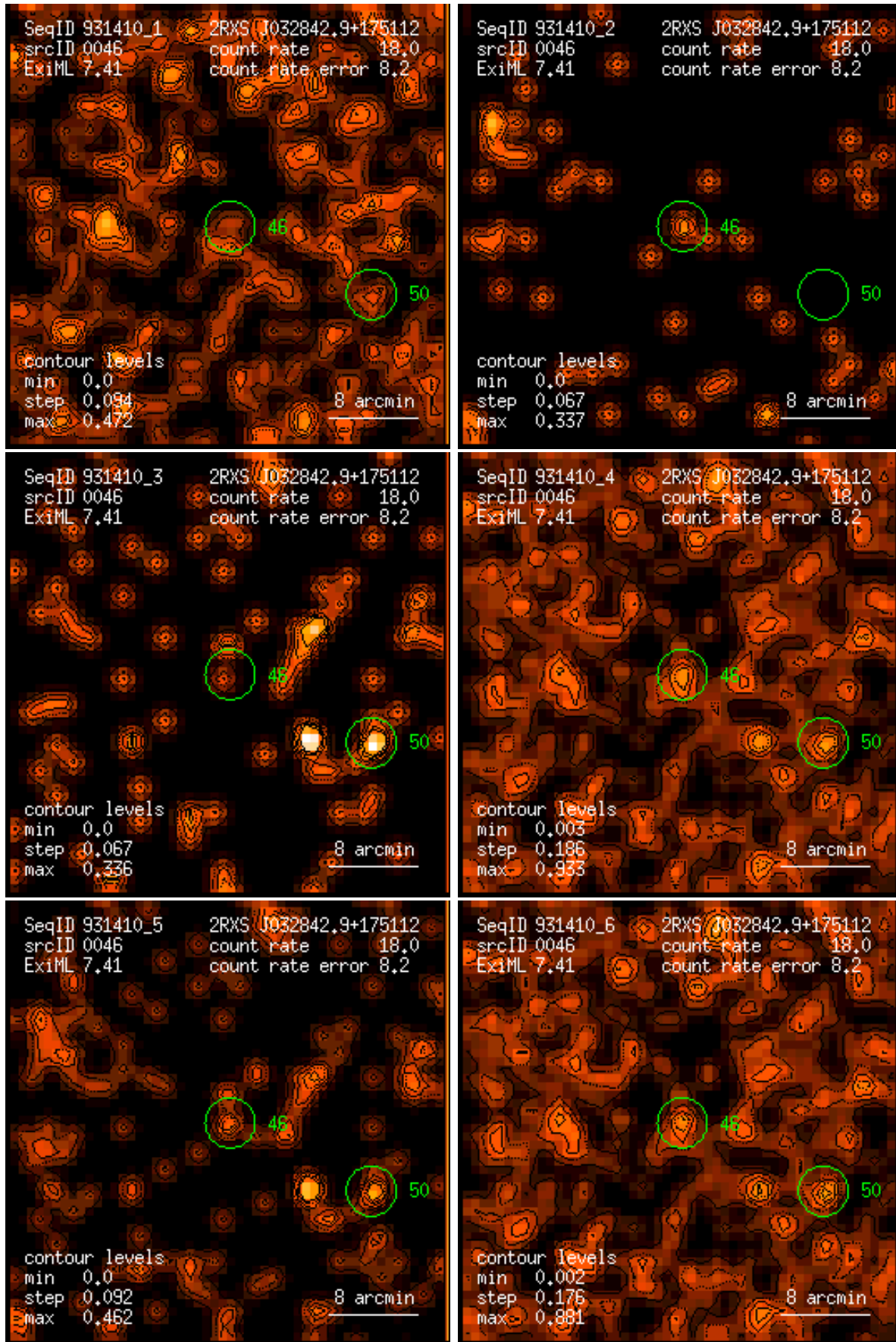
Figure 46: RASS 931410: detection 0046: band rate images, Gaussian filter: (1) PSPC channels 11 – 41, (2) 52 – 90, (3) 91 – 201, (4) 11 – 235, (5) 52 – 201, (6) 11 – 201. Broad band rates in counts/ks. Band rate contour levels in counts/ks/arcmin 2 .
