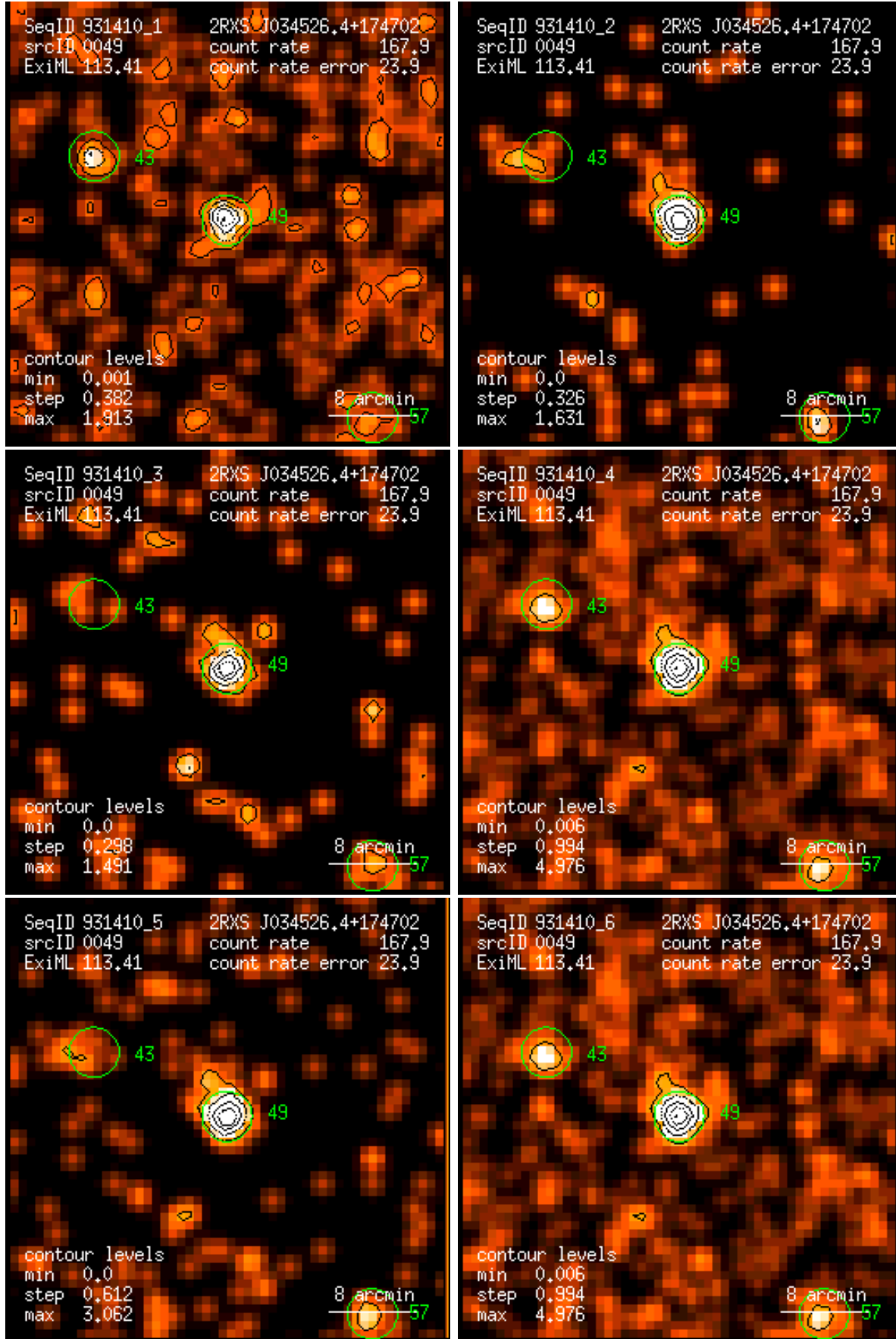
Figure 49: RASS 931410: detection 0049: band rate images, Gaussian filter: (1) PSPC channels 11 – 41, (2) 52 – 90, (3) 91 – 201, (4) 11 – 235, (5) 52 – 201, (6) 11 – 201. Broad band rates in counts/ks. Band rate contour levels in counts/ks/arcmin 2 .
