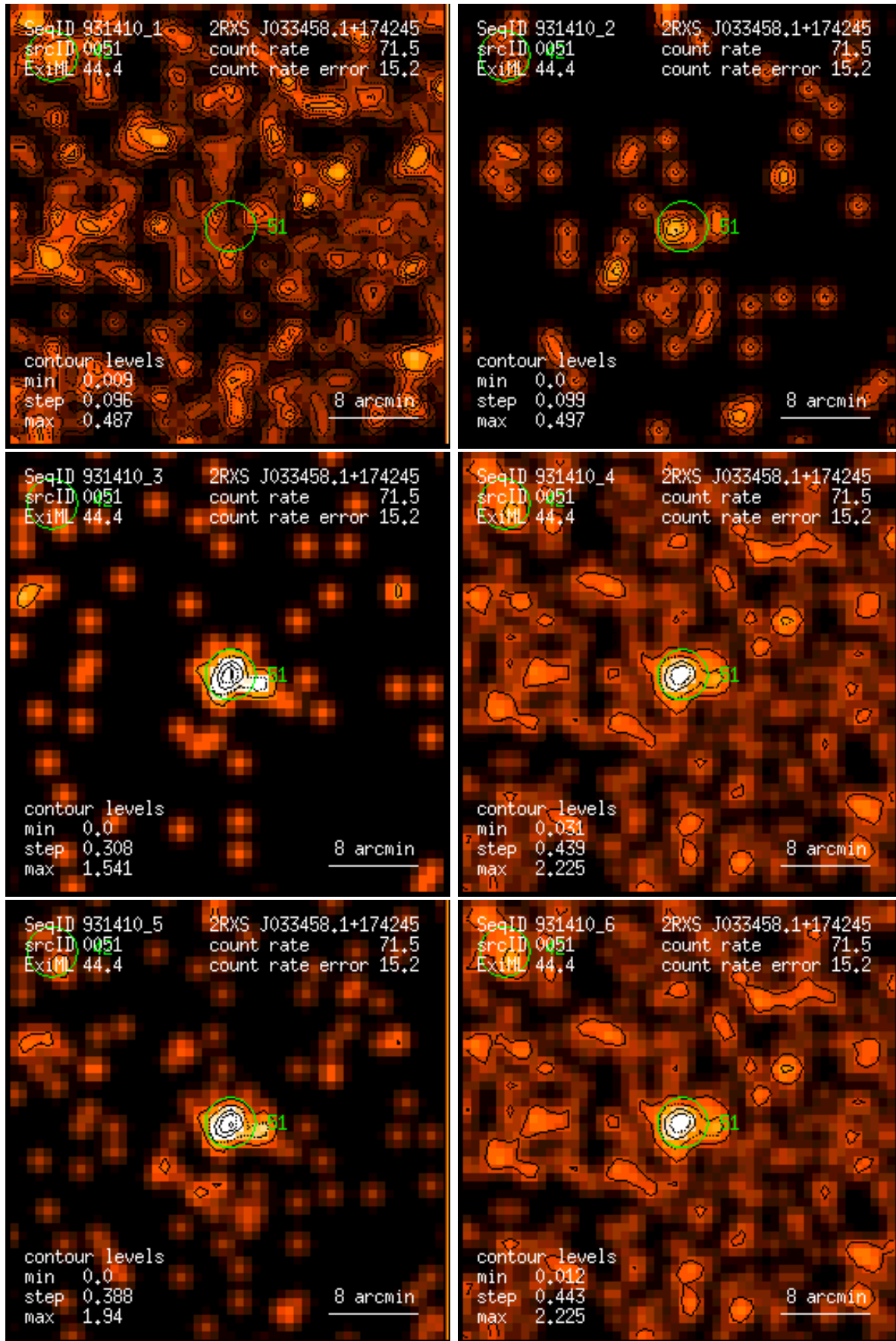
Figure 51: RASS 931410: detection 0051: band rate images, Gaussian filter: (1) PSPC channels 11 – 41, (2) 52 – 90, (3) 91 – 201, (4) 11 – 235, (5) 52 – 201, (6) 11 – 201. Broad band rates in counts/ks. Band rate contour levels in counts/ks/arcmin 2 .
