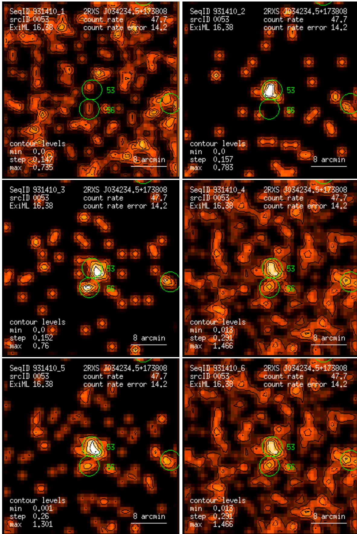
Figure 53: RASS 931410: detection 0053: band rate images, Gaussian filter: (1) PSPC channels 11 – 41, (2) 52 – 90, (3) 91 – 201, (4) 11 – 235, (5) 52 – 201, (6) 11 – 201. Broad band rates in counts/ks. Band rate contour levels in counts/ks/arcmin 2 .
