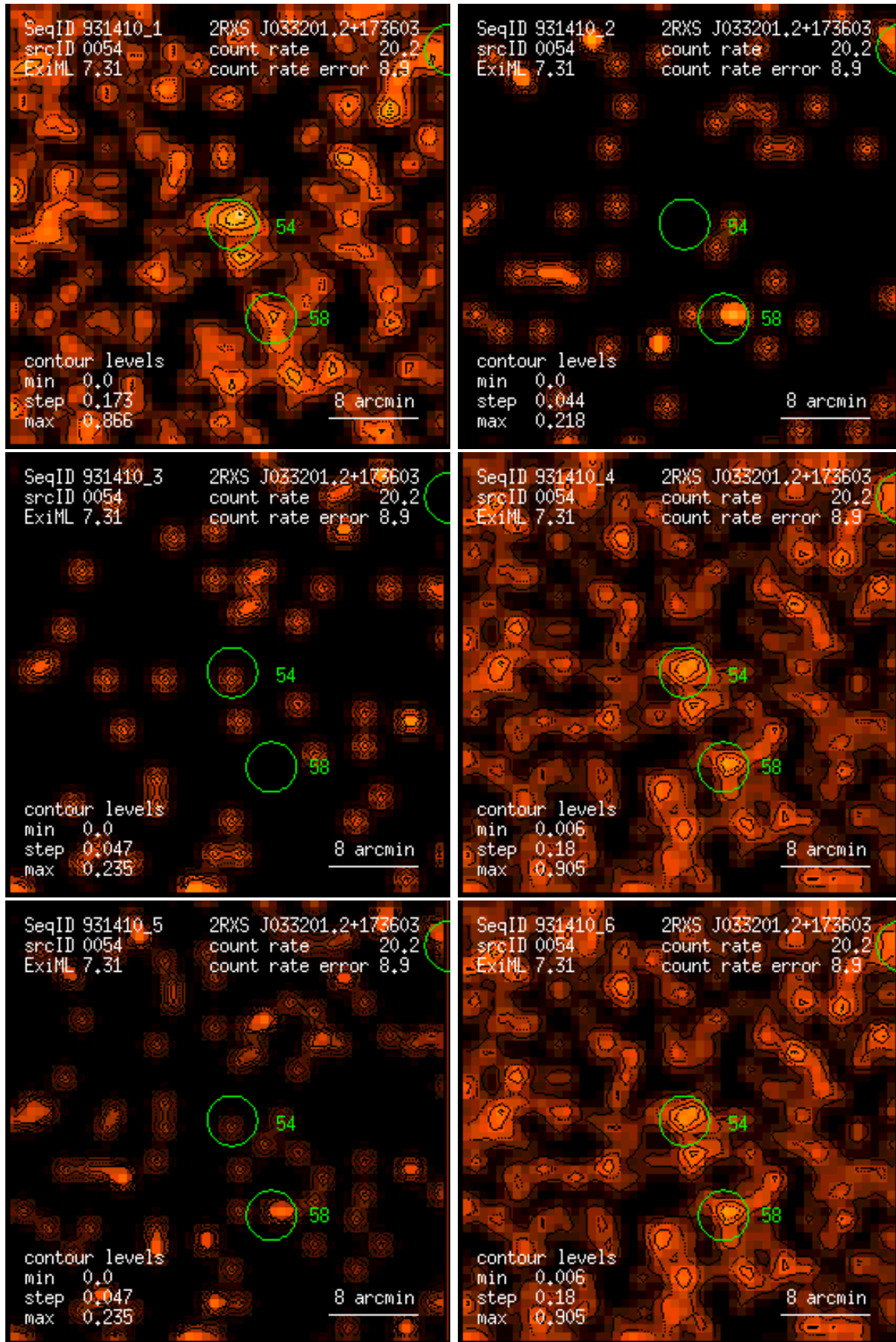
Figure 54: RASS 931410: detection 0054: band rate images, Gaussian filter: (1) PSPC channels 11 – 41, (2) 52 – 90, (3) 91 – 201, (4) 11 – 235, (5) 52 – 201, (6) 11 – 201. Broad band rates in counts/ks. Band rate contour levels in counts/ks/arcmin 2 .
