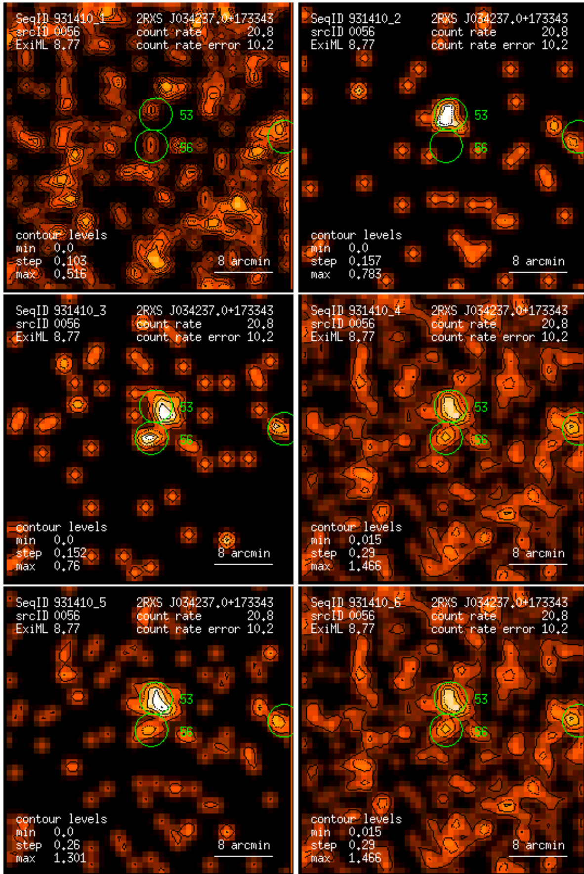
Figure 56: RASS 931410: detection 0056: band rate images, Gaussian filter: (1) PSPC channels 11 – 41, (2) 52 – 90, (3) 91 – 201, (4) 11 – 235, (5) 52 – 201, (6) 11 – 201. Broad band rates in counts/ks. Band rate contour levels in counts/ks/arcmin 2 .
