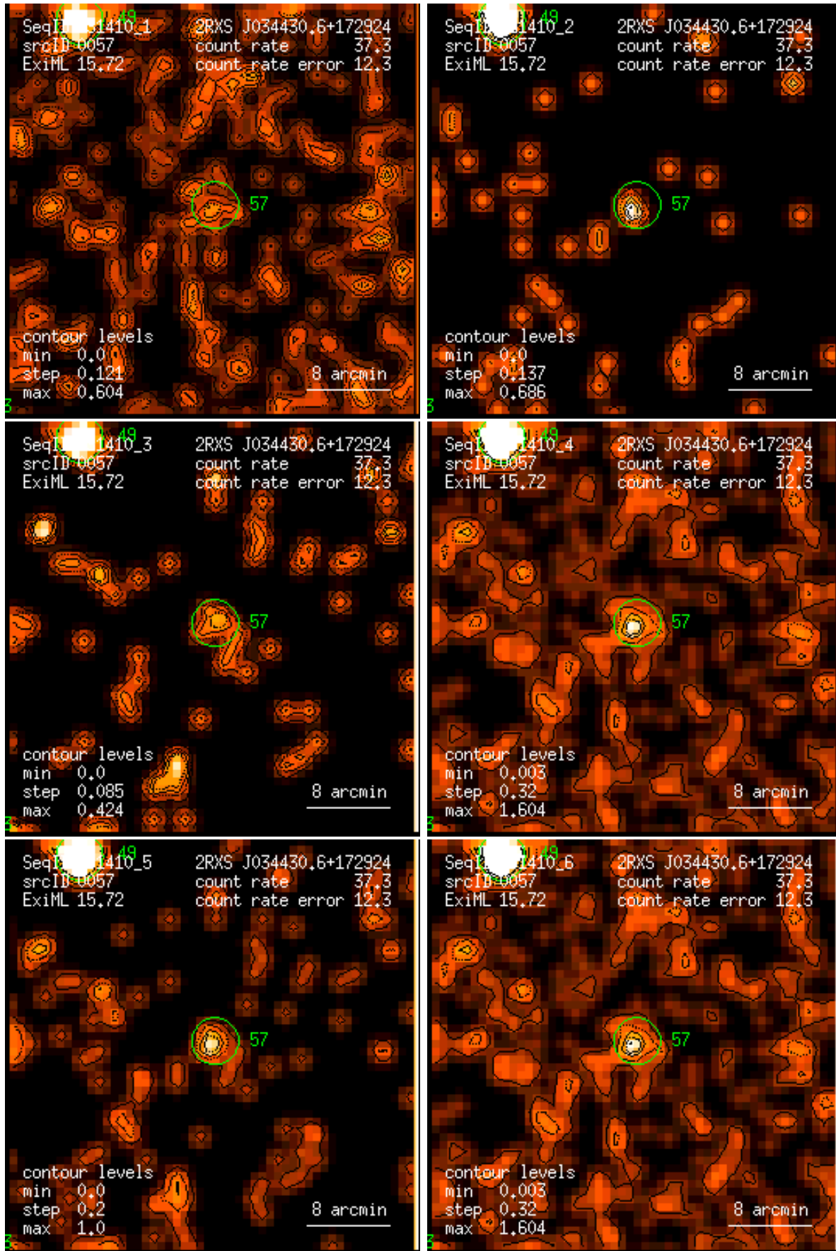
Figure 57: RASS 931410: detection 0057: band rate images, Gaussian filter: (1) PSPC channels 11 – 41, (2) 52 – 90, (3) 91 – 201, (4) 11 – 235, (5) 52 – 201, (6) 11 – 201. Broad band rates in counts/ks. Band rate contour levels in counts/ks/arcmin 2 .
