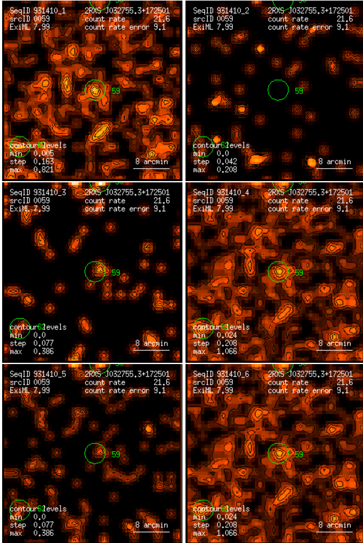
Figure 59: RASS 931410: detection 0059: band rate images, Gaussian filter: (1) PSPC channels 11 – 41, (2) 52 – 90, (3) 91 – 201, (4) 11 – 235, (5) 52 – 201, (6) 11 – 201. Broad band rates in counts/ks. Band rate contour levels in counts/ks/arcmin 2 .
