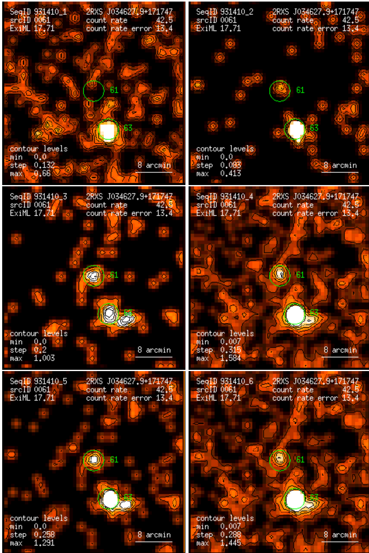
Figure 61: RASS 931410: detection 0061: band rate images, Gaussian filter: (1) PSPC channels 11 – 41, (2) 52 – 90, (3) 91 – 201, (4) 11 – 235, (5) 52 – 201, (6) 11 – 201. Broad band rates in counts/ks. Band rate contour levels in counts/ks/arcmin 2 .
