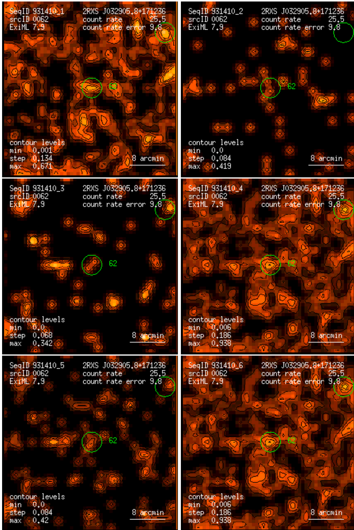
Figure 62: RASS 931410: detection 0062: band rate images, Gaussian filter: (1) PSPC channels 11 – 41, (2) 52 – 90, (3) 91 – 201, (4) 11 – 235, (5) 52 – 201, (6) 11 – 201. Broad band rates in counts/ks. Band rate contour levels in counts/ks/arcmin 2 .
