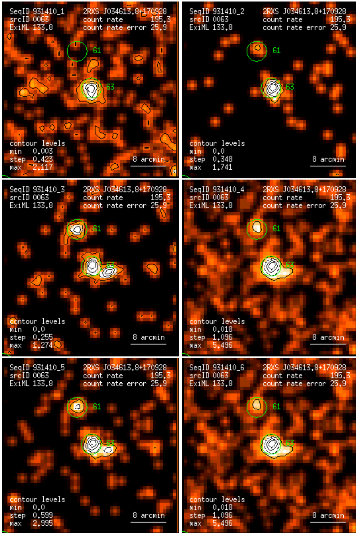
Figure 63: RASS 931410: detection 0063: band rate images, Gaussian filter: (1) PSPC channels 11 – 41, (2) 52 – 90, (3) 91 – 201, (4) 11 – 235, (5) 52 – 201, (6) 11 – 201. Broad band rates in counts/ks. Band rate contour levels in counts/ks/arcmin 2 .
