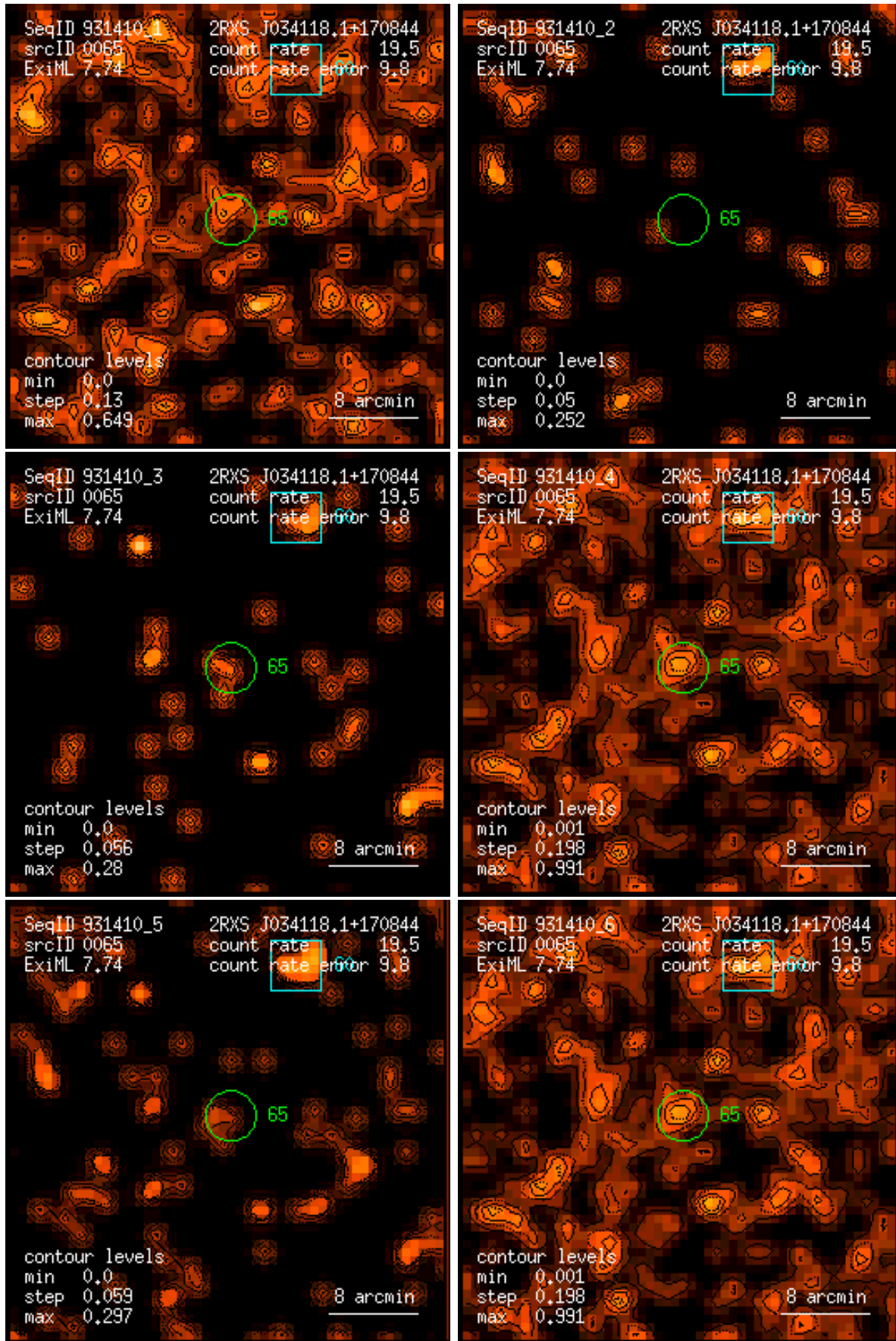
Figure 65: RASS 931410: detection 0065: band rate images, Gaussian filter: (1) PSPC channels 11 – 41, (2) 52 – 90, (3) 91 – 201, (4) 11 – 235, (5) 52 – 201, (6) 11 – 201. Broad band rates in counts/ks. Band rate contour levels in counts/ks/arcmin 2 .
