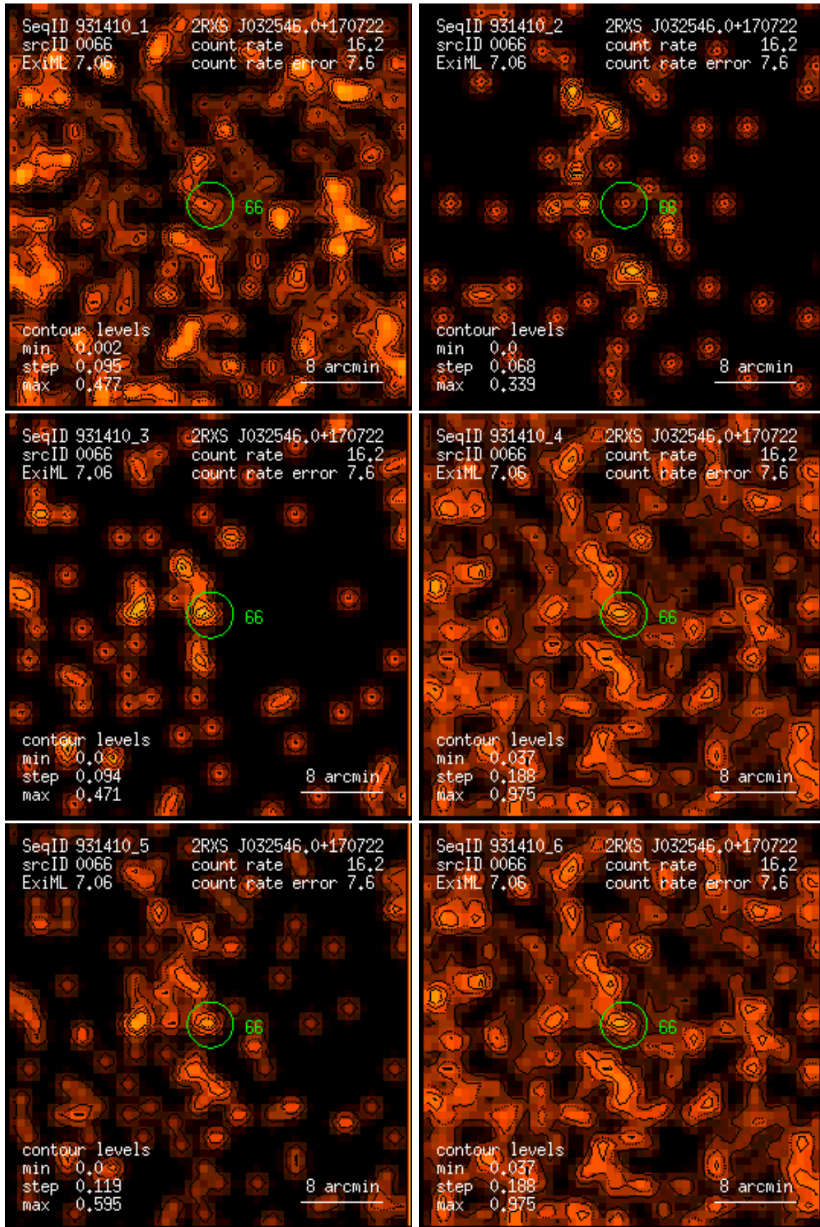
Figure 66: RASS 931410: detection 0066: band rate images, Gaussian filter: (1) PSPC channels 11 – 41, (2) 52 – 90, (3) 91 – 201, (4) 11 – 235, (5) 52 – 201, (6) 11 – 201. Broad band rates in counts/ks. Band rate contour levels in counts/ks/arcmin 2 .
