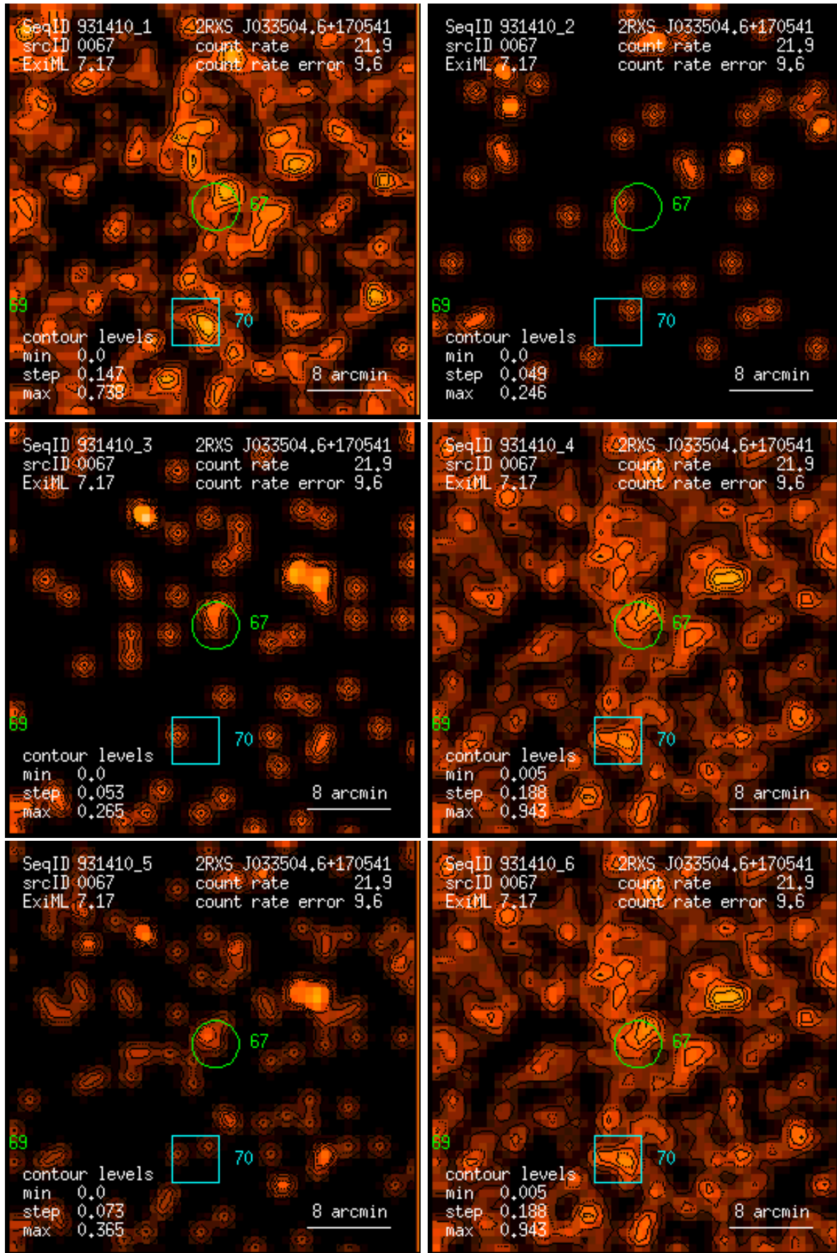
Figure 67: RASS 931410: detection 0067: band rate images, Gaussian filter: (1) PSPC channels 11 – 41, (2) 52 – 90, (3) 91 – 201, (4) 11 – 235, (5) 52 – 201, (6) 11 – 201. Broad band rates in counts/ks. Band rate contour levels in counts/ks/arcmin 2 .
