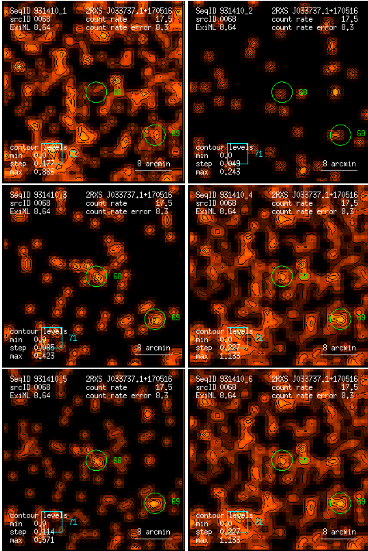
Figure 68: RASS 931410: detection 0068: band rate images, Gaussian filter: (1) PSPC channels 11 – 41, (2) 52 – 90, (3) 91 – 201, (4) 11 – 235, (5) 52 – 201, (6) 11 – 201. Broad band rates in counts/ks. Band rate contour levels in counts/ks/arcmin 2 .
