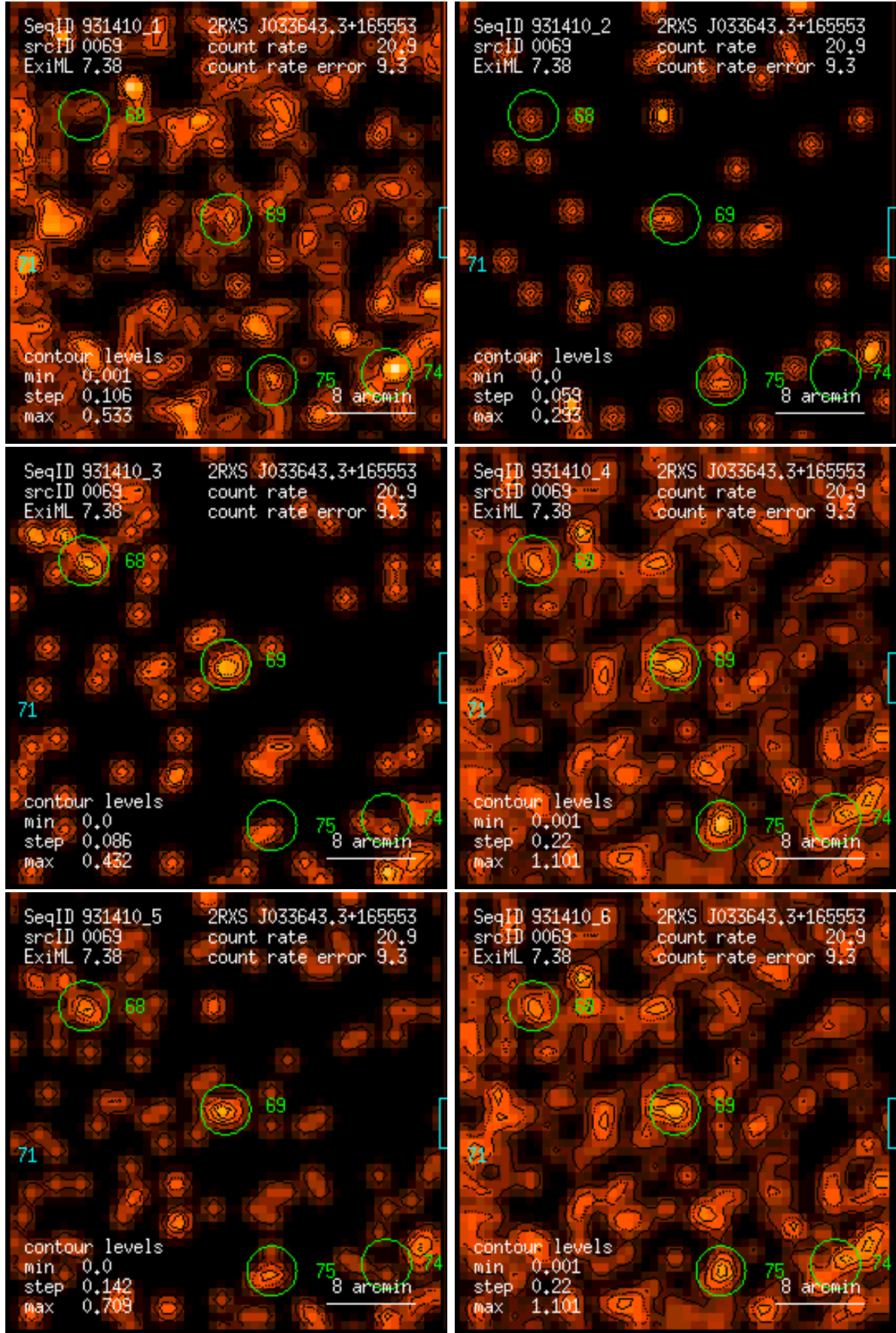
Figure 69: RASS 931410: detection 0069: band rate images, Gaussian filter: (1) PSPC channels 11 – 41, (2) 52 – 90, (3) 91 – 201, (4) 11 – 235, (5) 52 – 201, (6) 11 – 201. Broad band rates in counts/ks. Band rate contour levels in counts/ks/arcmin 2 .
