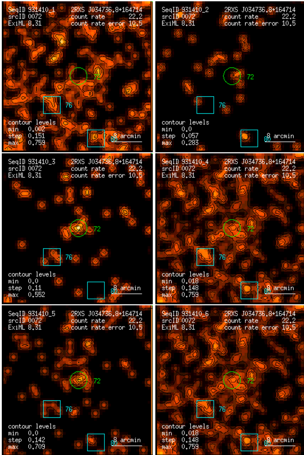
Figure 72: RASS 931410: detection 0072: band rate images, Gaussian filter: (1) PSPC channels 11 – 41, (2) 52 – 90, (3) 91 – 201, (4) 11 – 235, (5) 52 – 201, (6) 11 – 201. Broad band rates in counts/ks. Band rate contour levels in counts/ks/arcmin 2 .
