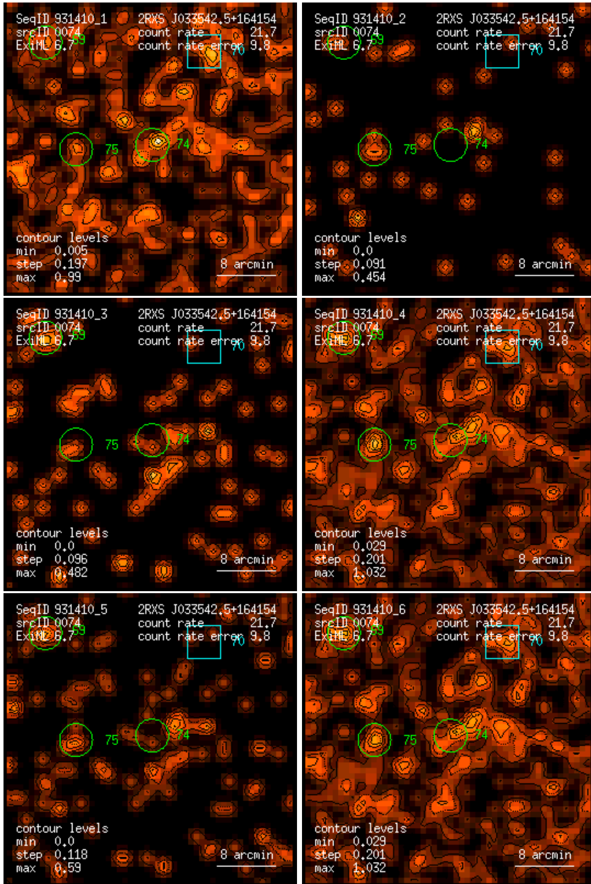
Figure 74: RASS 931410: detection 0074: band rate images, Gaussian filter: (1) PSPC channels 11 – 41, (2) 52 – 90, (3) 91 – 201, (4) 11 – 235, (5) 52 – 201, (6) 11 – 201. Broad band rates in counts/ks. Band rate contour levels in counts/ks/arcmin 2 .
