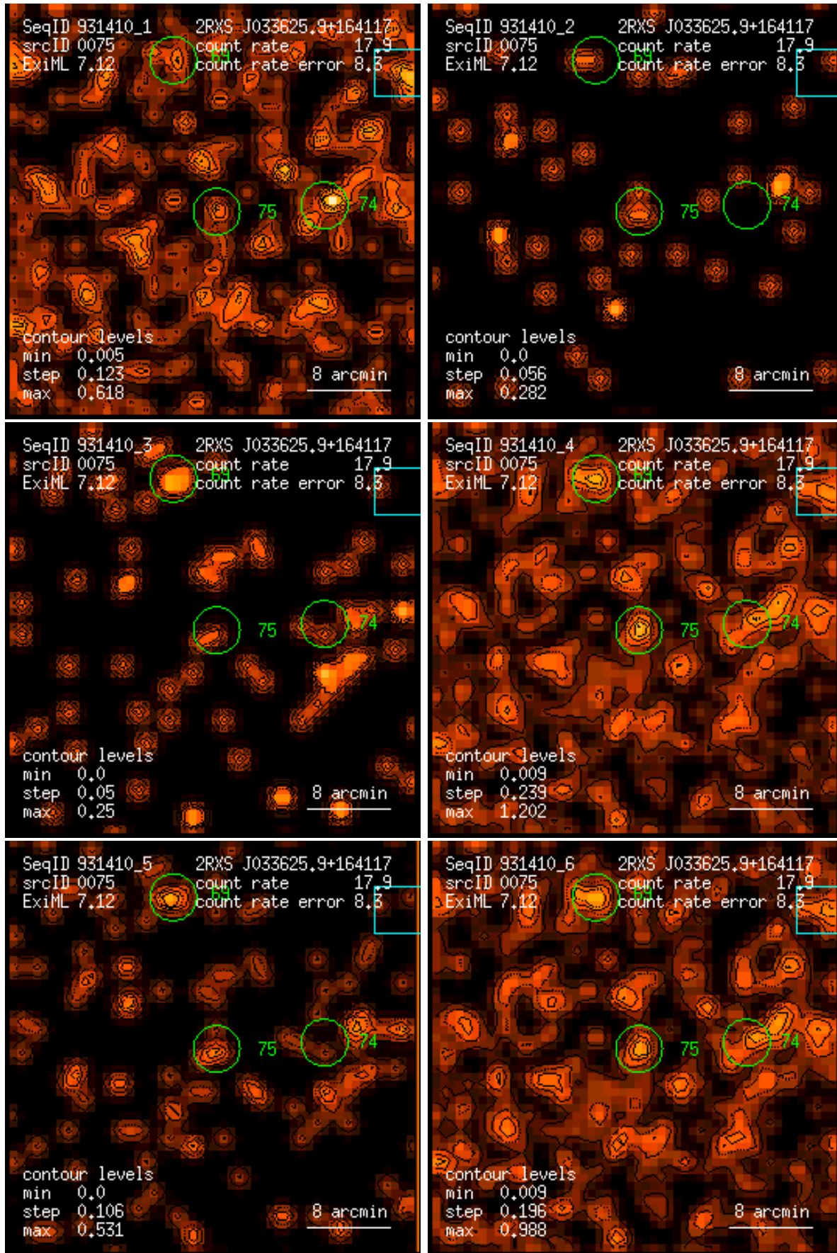
Figure 75: RASS 931410: detection 0075: band rate images, Gaussian filter: (1) PSPC channels 11 – 41, (2) 52 – 90, (3) 91 – 201, (4) 11 – 235, (5) 52 – 201, (6) 11 – 201. Broad band rates in counts/ks. Band rate contour levels in counts/ks/arcmin 2 .
