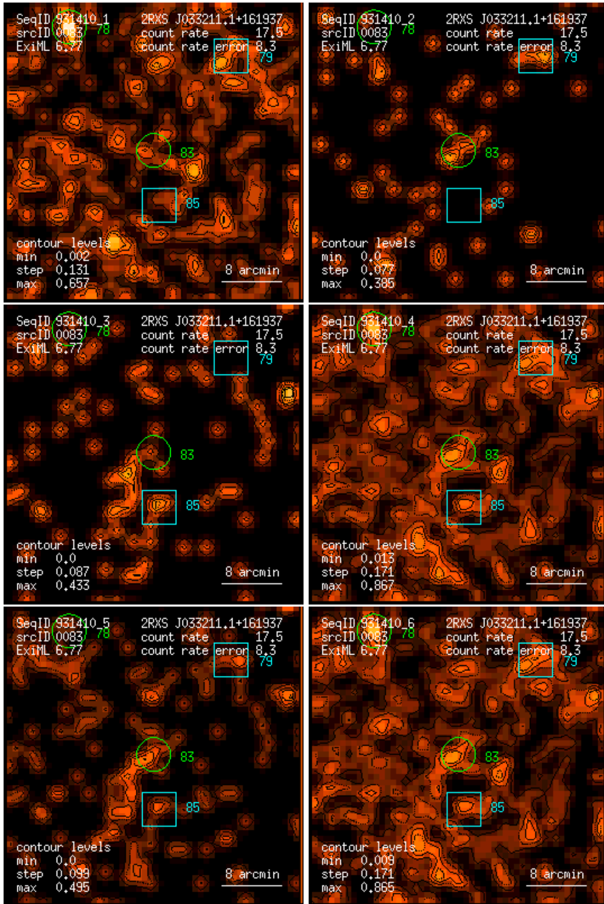
Figure 83: RASS 931410: detection 0083: band rate images, Gaussian filter: (1) PSPC channels 11 – 41, (2) 52 – 90, (3) 91 – 201, (4) 11 – 235, (5) 52 – 201, (6) 11 – 201. Broad band rates in counts/ks. Band rate contour levels in counts/ks/arcmin 2 .
