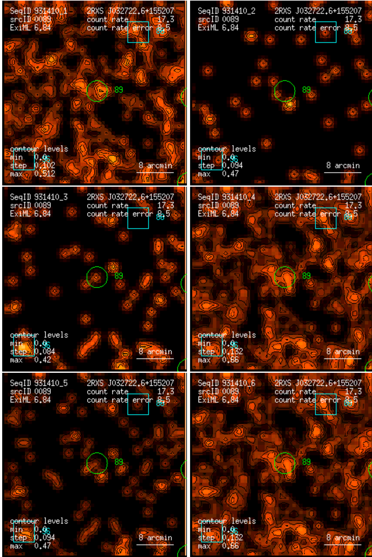
Figure 89: RASS 931410: detection 0089: band rate images, Gaussian filter: (1) PSPC channels 11 – 41, (2) 52 – 90, (3) 91 – 201, (4) 11 – 235, (5) 52 – 201, (6) 11 – 201. Broad band rates in counts/ks. Band rate contour levels in counts/ks/arcmin 2 .
