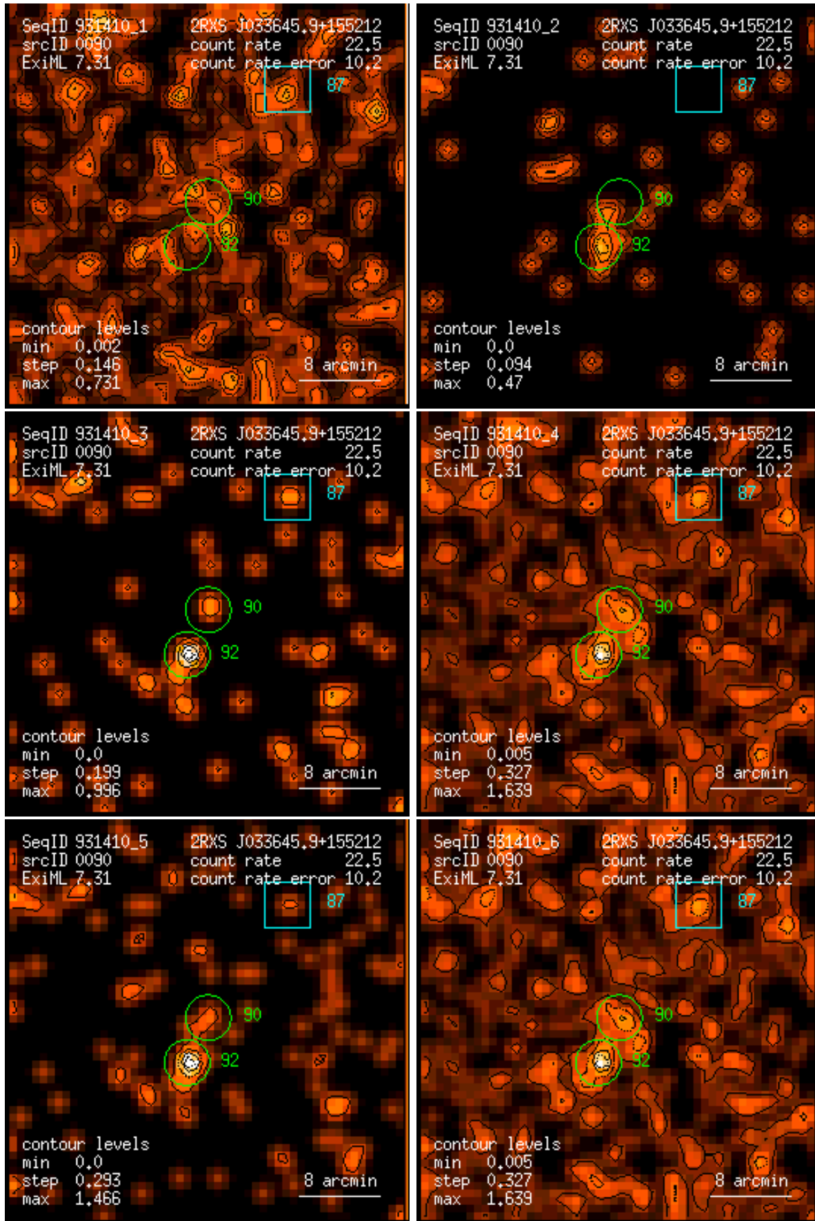
Figure 90: RASS 931410: detection 0090: band rate images, Gaussian filter: (1) PSPC channels 11 – 41, (2) 52 – 90, (3) 91 – 201, (4) 11 – 235, (5) 52 – 201, (6) 11 – 201. Broad band rates in counts/ks. Band rate contour levels in counts/ks/arcmin 2 .
