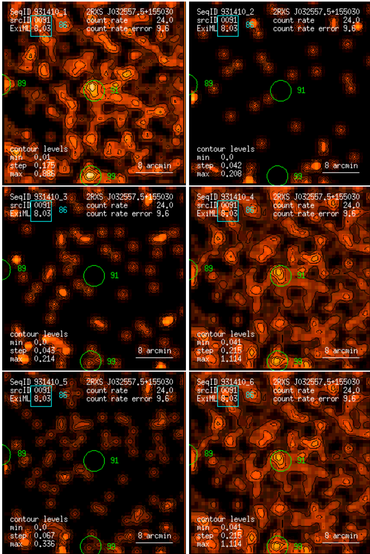
Figure 91: RASS 931410: detection 0091: band rate images, Gaussian filter: (1) PSPC channels 11 – 41, (2) 52 – 90, (3) 91 – 201, (4) 11 – 235, (5) 52 – 201, (6) 11 – 201. Broad band rates in counts/ks. Band rate contour levels in counts/ks/arcmin 2 .
