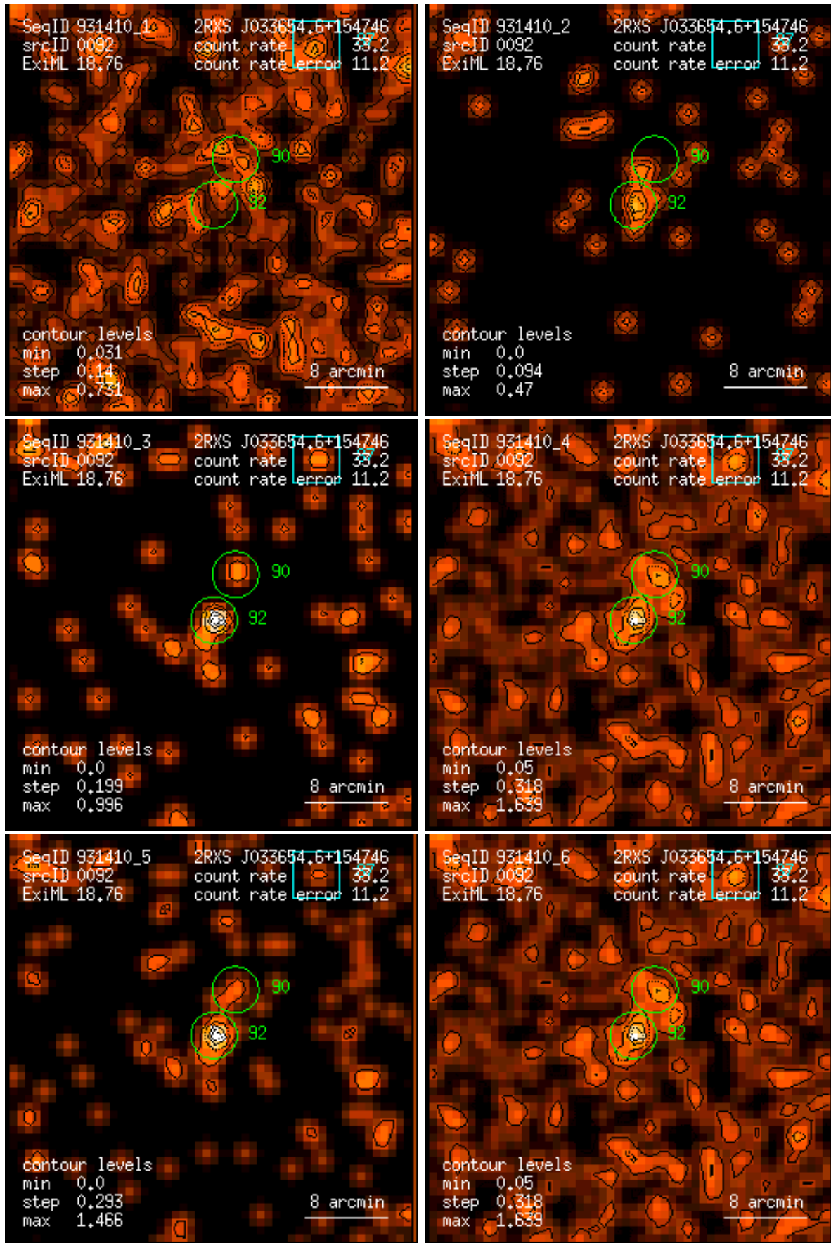
Figure 92: RASS 931410: detection 0092: band rate images, Gaussian filter: (1) PSPC channels 11 – 41, (2) 52 – 90, (3) 91 – 201, (4) 11 – 235, (5) 52 – 201, (6) 11 – 201. Broad band rates in counts/ks. Band rate contour levels in counts/ks/arcmin 2 .
