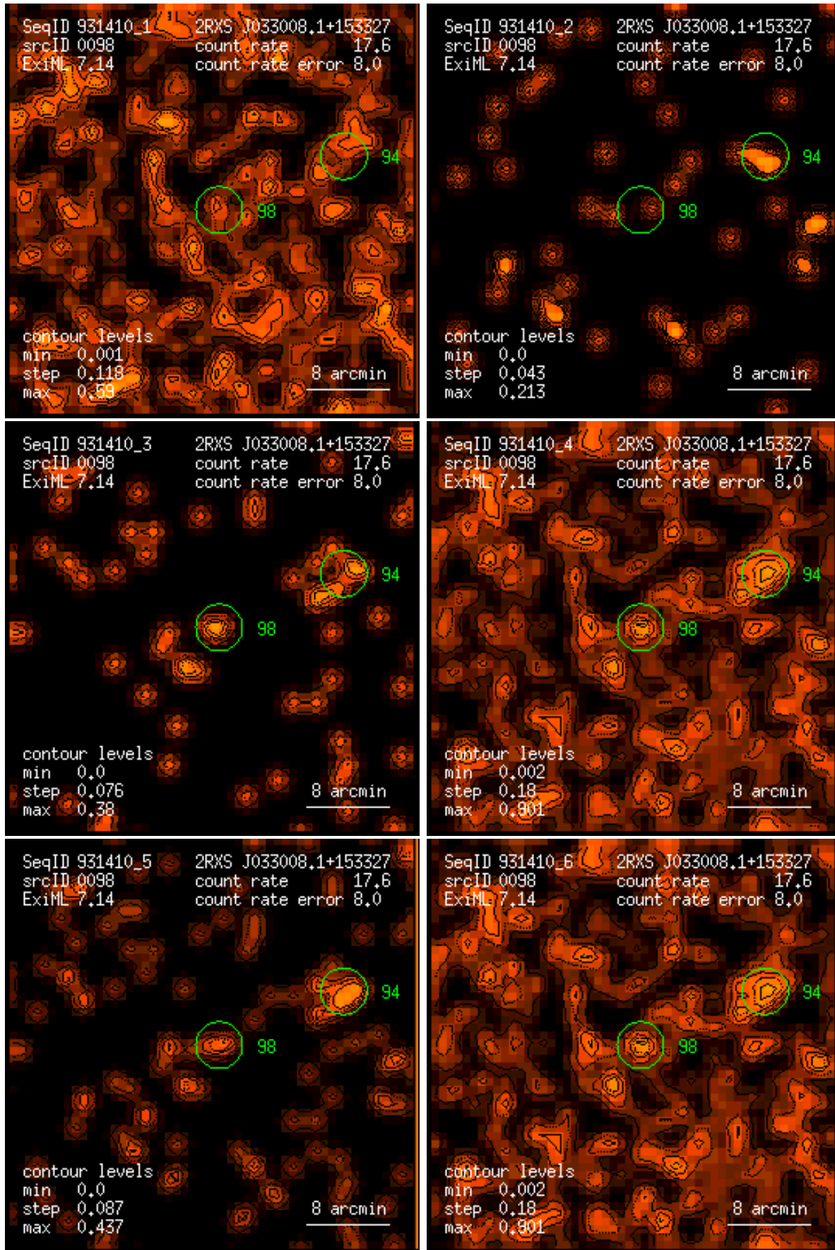
Figure 98: RASS 931410: detection 0098: band rate images, Gaussian filter: (1) PSPC channels 11 – 41, (2) 52 – 90, (3) 91 – 201, (4) 11 – 235, (5) 52 – 201, (6) 11 – 201. Broad band rates in counts/ks. Band rate contour levels in counts/ks/arcmin 2 .
