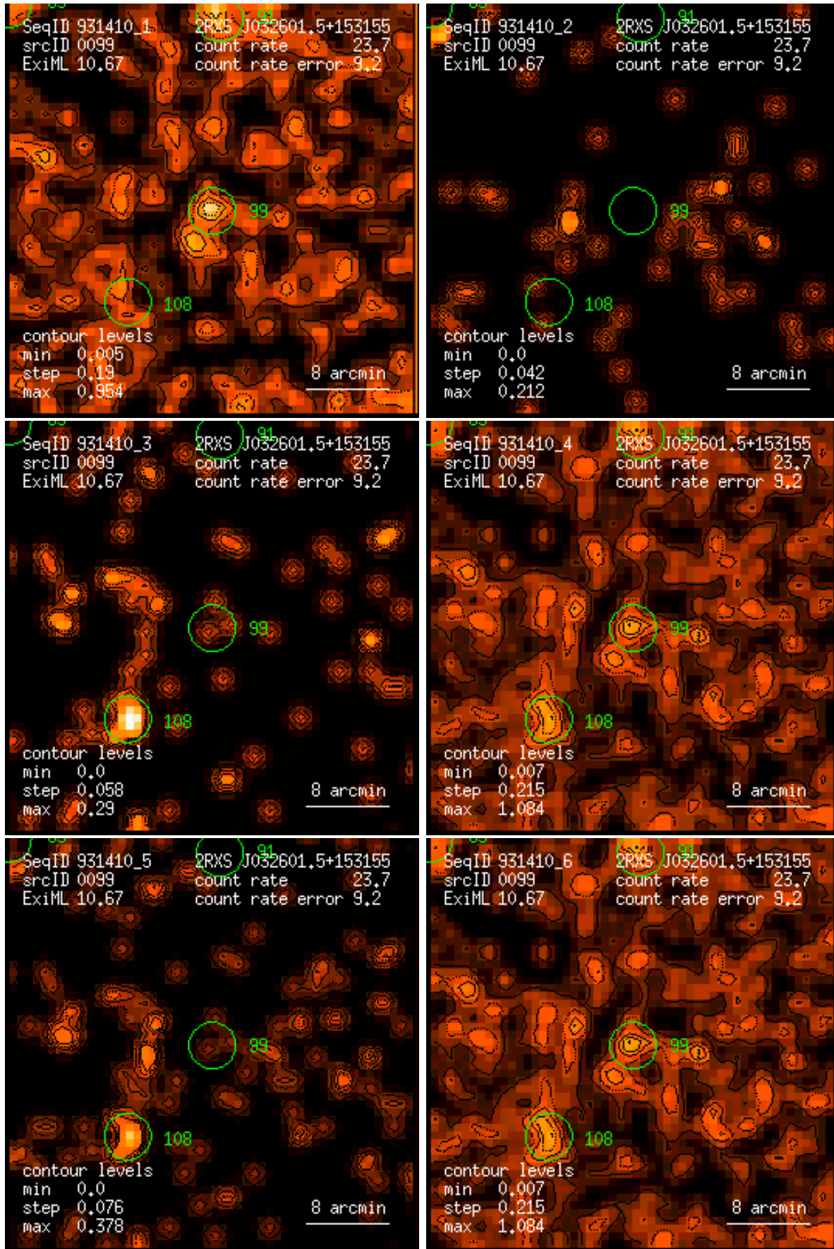
Figure 99: RASS 931410: detection 0099: band rate images, Gaussian filter: (1) PSPC channels 11 – 41, (2) 52 – 90, (3) 91 – 201, (4) 11 – 235, (5) 52 – 201, (6) 11 – 201. Broad band rates in counts/ks. Band rate contour levels in counts/ks/arcmin 2 .
