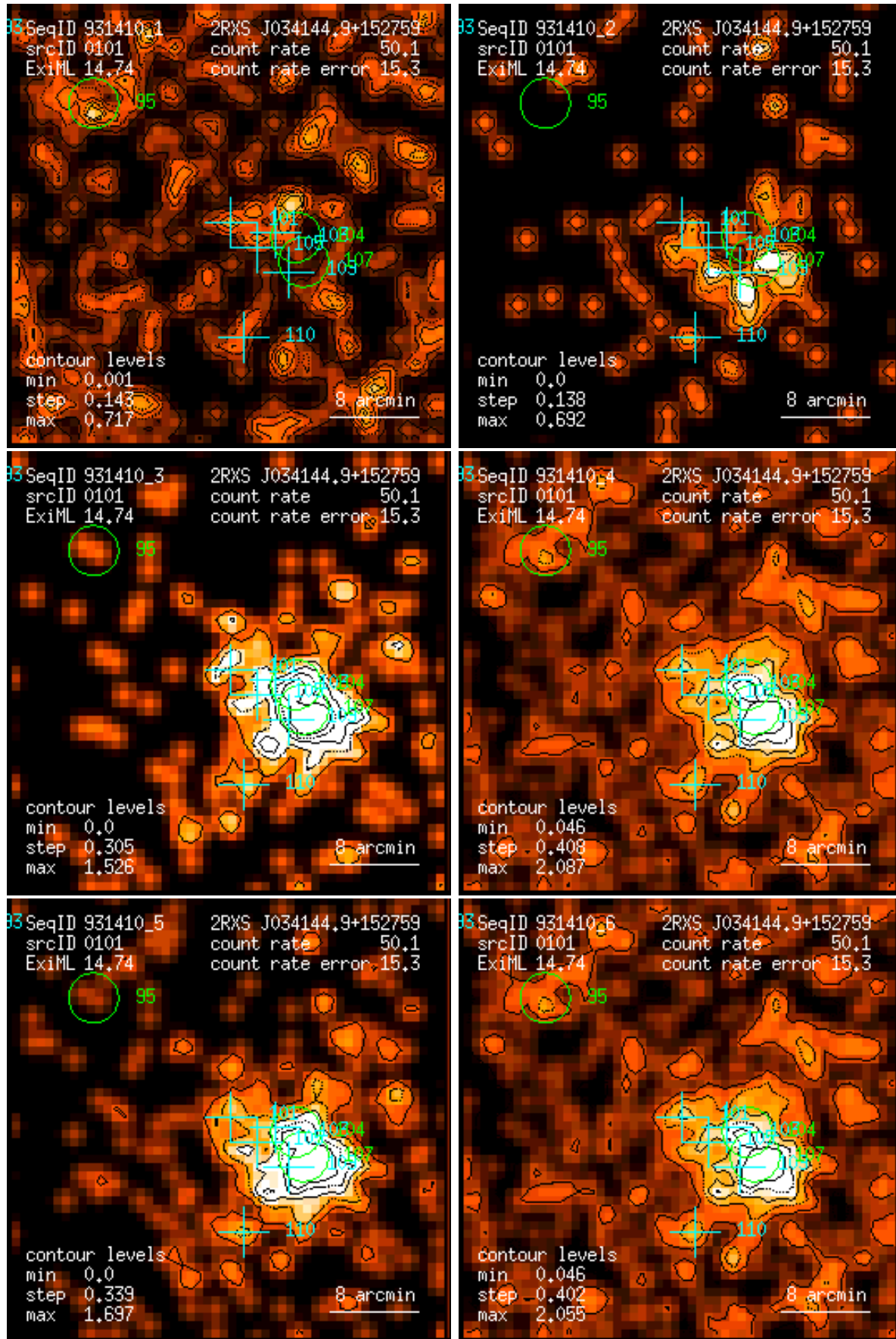
Figure 101: RASS 931410: detection 0101: band rate images, Gaussian filter: (1) PSPC channels 11 – 41, (2) 52 – 90, (3) 91 – 201, (4) 11 – 235, (5) 52 – 201, (6) 11 – 201. Broad band rates in counts/ks. Band rate contour levels in counts/ks/arcmin 2 .
