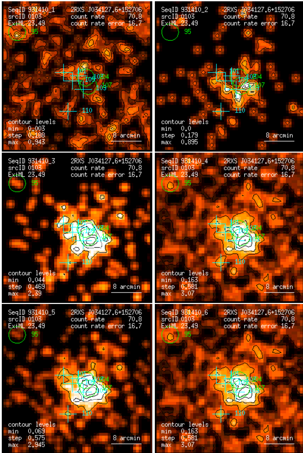
Figure 103: RASS 931410: detection 0103: band rate images, Gaussian filter: (1) PSPC channels 11 – 41, (2) 52 – 90, (3) 91 – 201, (4) 11 – 235, (5) 52 – 201, (6) 11 – 201. Broad band rates in counts/ks. Band rate contour levels in counts/ks/arcmin 2 .
