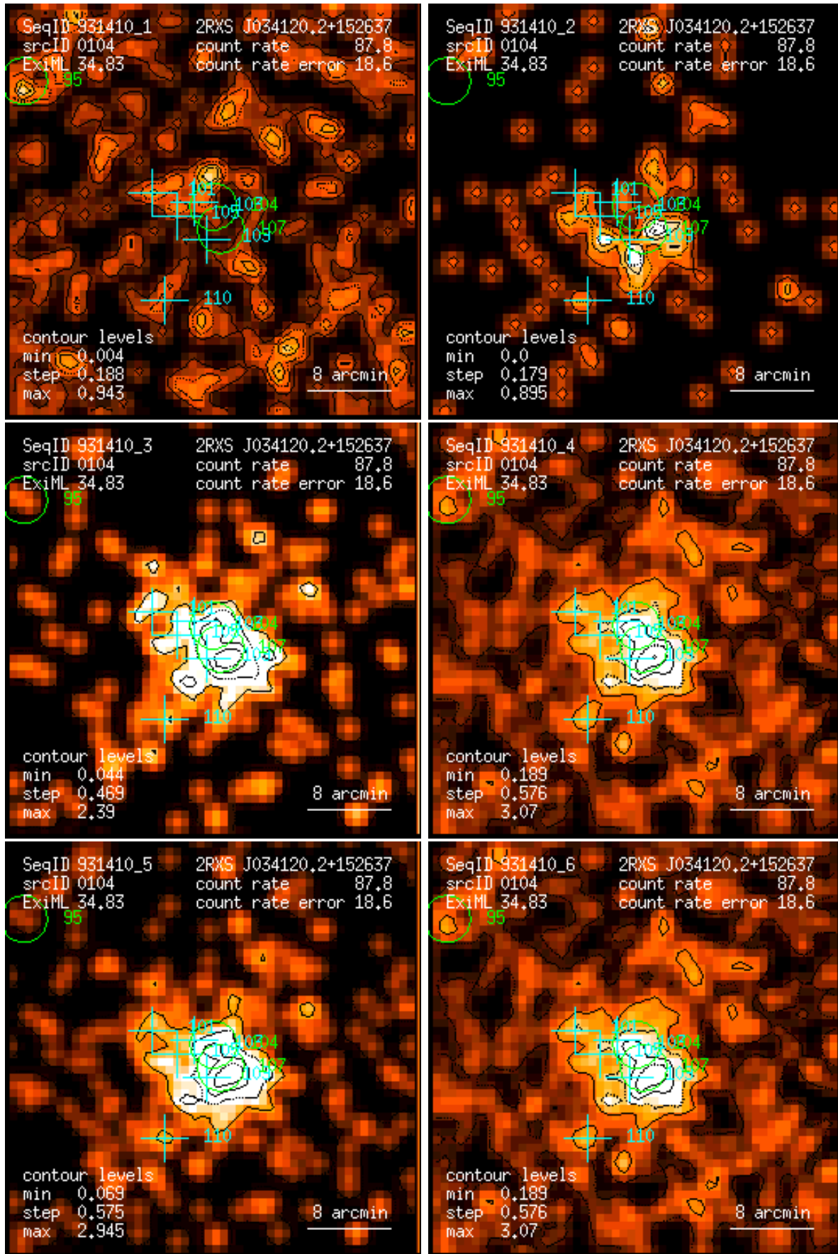
Figure 104: RASS 931410: detection 0104: band rate images, Gaussian filter: (1) PSPC channels 11 – 41, (2) 52 – 90, (3) 91 – 201, (4) 11 – 235, (5) 52 – 201, (6) 11 – 201. Broad band rates in counts/ks. Band rate contour levels in counts/ks/arcmin 2 .
