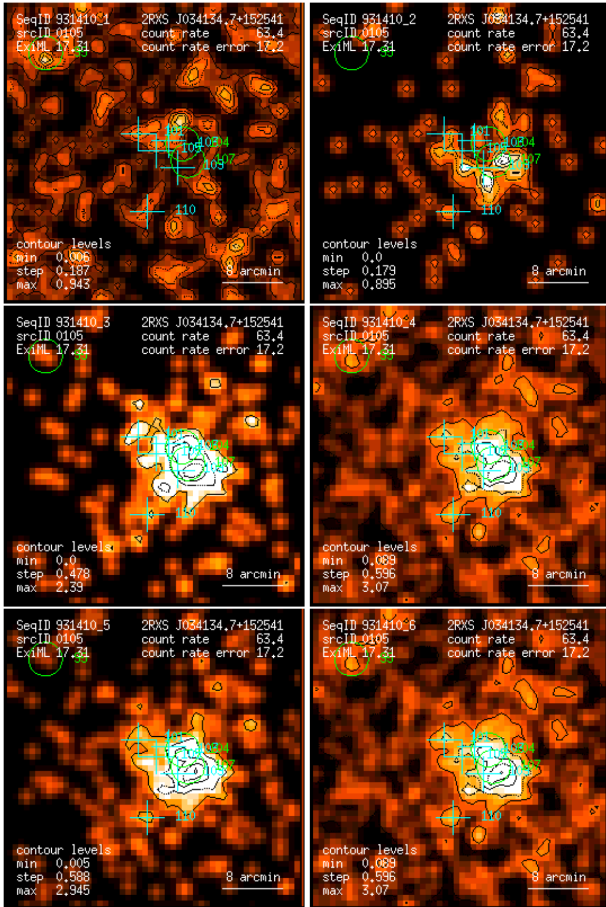
Figure 105: RASS 931410: detection 0105: band rate images, Gaussian filter: (1) PSPC channels 11 – 41, (2) 52 – 90, (3) 91 – 201, (4) 11 – 235, (5) 52 – 201, (6) 11 – 201. Broad band rates in counts/ks. Band rate contour levels in counts/ks/arcmin 2 .
