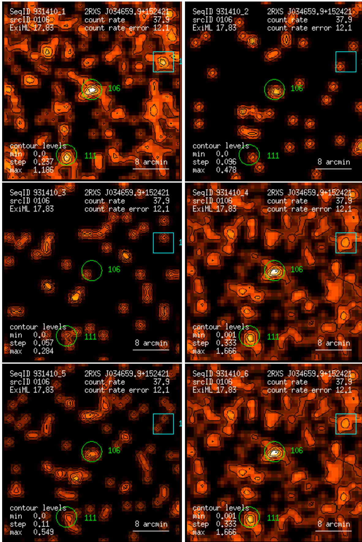
Figure 106: RASS 931410: detection 0106: band rate images, Gaussian filter: (1) PSPC channels 11 – 41, (2) 52 – 90, (3) 91 – 201, (4) 11 – 235, (5) 52 – 201, (6) 11 – 201. Broad band rates in counts/ks. Band rate contour levels in counts/ks/arcmin 2 .
