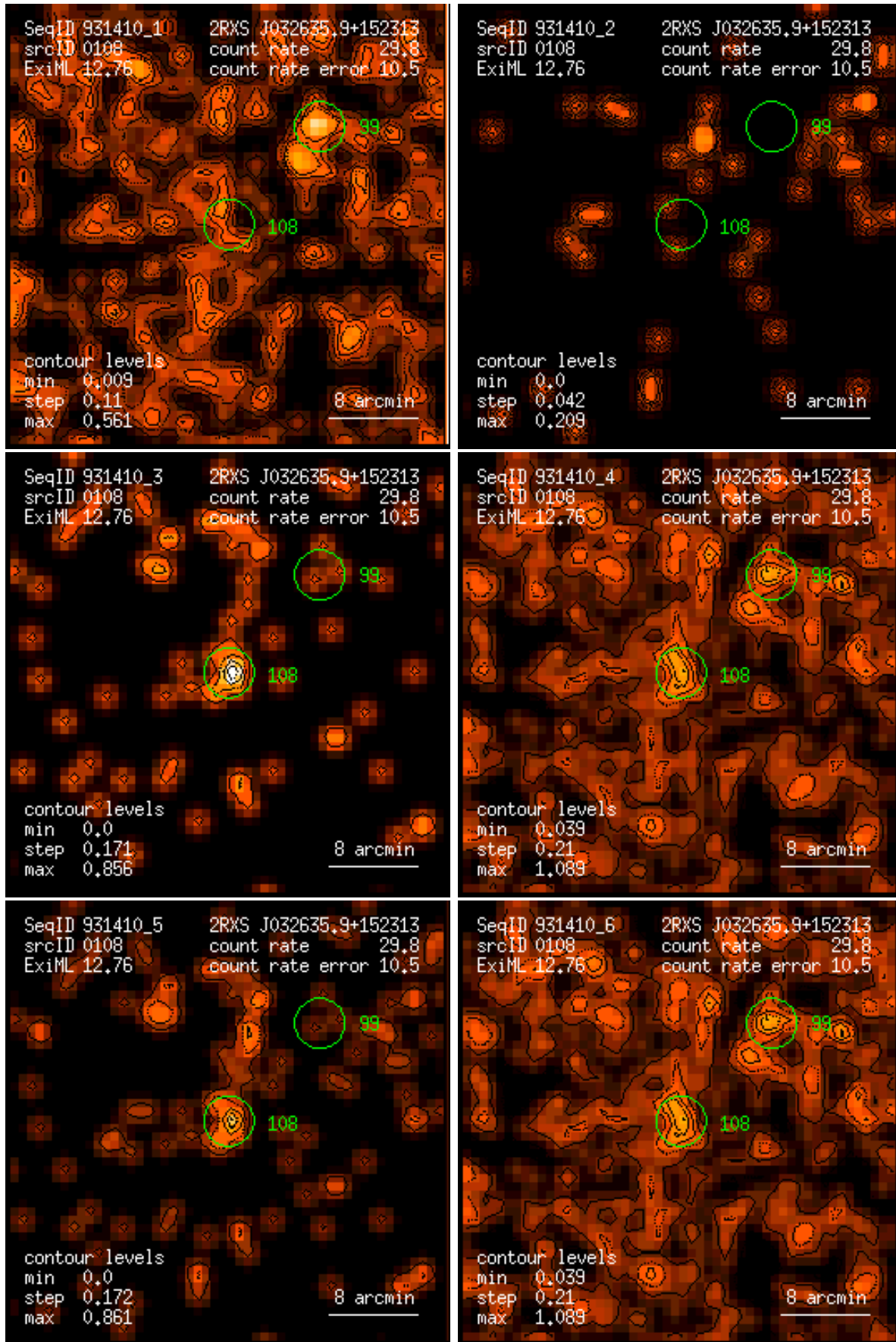
Figure 108: RASS 931410: detection 0108: band rate images, Gaussian filter: (1) PSPC channels 11 – 41, (2) 52 – 90, (3) 91 – 201, (4) 11 – 235, (5) 52 – 201, (6) 11 – 201. Broad band rates in counts/ks. Band rate contour levels in counts/ks/arcmin 2 .
